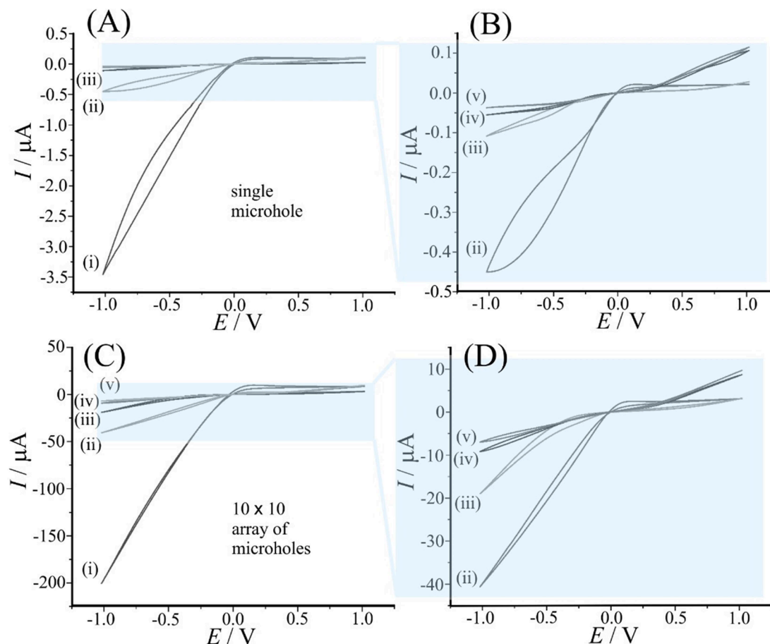
Fig. 2. (A,B) Cyclic voltammety data (scan rate 0.2 \text{ Vs}^{-1} ) for a 10 \mu\text{m} microhole covered with PIM-EA-TB and immersed in aqueous 10 mM NaCl at various pH values: (i) 2, (ii) 3, (iii) 4, (iv) 5, and (v) 6. (C,D) as before but for a 10 \times 10 array of microholes.
