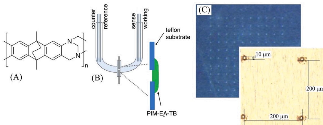
Fig. 1. (A) Molecular structure of PIM-EA-TB. (B) Four-electrode membrane voltammetry experimental configuration. (C) Optical micrographs showing the 10 × 10 microhole array and individual microholes with 10 μm diameter and 200 μm pitch in a Teflon substrate 5 μm thick.
