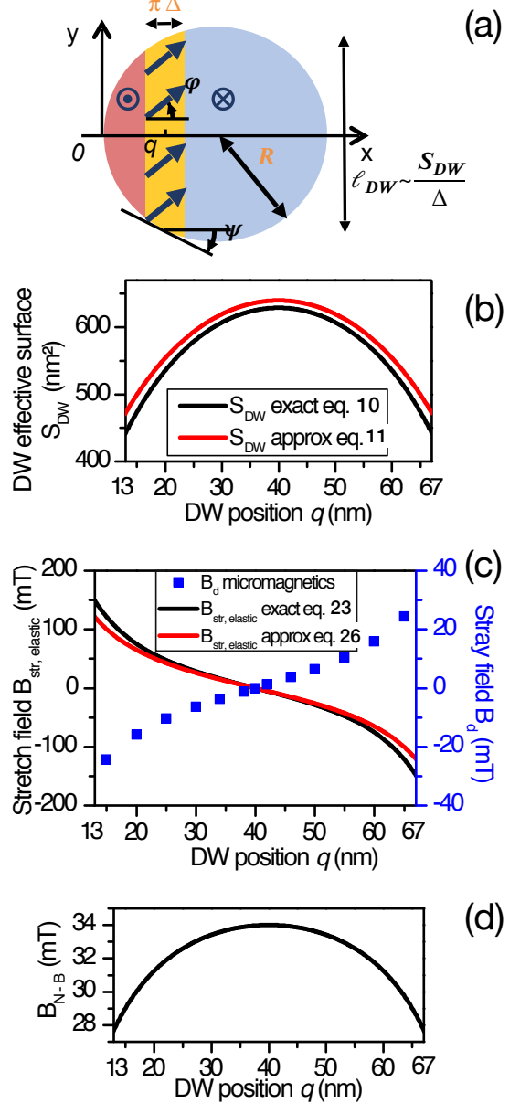
FIG. 7. (a) Sketch of the geometry and main definitions. (b) Effective surface S_{\text{DW}}(q) of a straight domain wall in an 80 nm disc as computed exactly using Eq. 10 and as approximated using the product of the length of the chord by \Delta . (c) Elastic part of the stretch field (Eq. 23 and its large diameter approximation when confusing the wall length and the disc chord, as performed in Eq. 26) and stray field H_d(q) of the two domains versus DW position in an 80 nm disc. (d) Domain wall stiffness field H_{N \leftrightarrow B}(q) versus DW position in an 80 nm disc.
