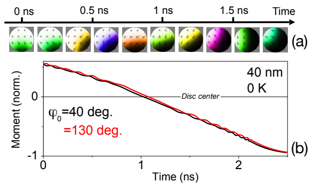
FIG. 4. Micromagnetic simulations of the DW dynamics within a 40-nm disc for a wall with optimal initial curvature. a) Snapshots of an initial magnetization state with \{\phi_0, q_0\} = \{40 \text{ deg.}, 10 \text{ nm}\} and its subsequent evolution under an applied voltage equal to V_c . b) Resulting evolution of the spatial average of the m_z component of the magnetization for the same simulation and for one with an initial tilt angle incremented by 90 degrees.
