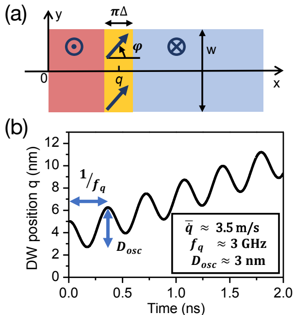
FIG. 6. Dynamics of a domain wall in an infinitely long stripe in the q - \phi model. (a) Geometry: a straight wall (yellow) of width \pi\Delta and of tilt \phi is at a position q within a stripe of width w . (b) Domain wall position as a function of time for a spin-torque \sigma j = 0.5 GHz, an applied field \mu_0 H_z = 50 mT and material parameters modeling a CoFeB free layer with perpendicular anisotropy.
