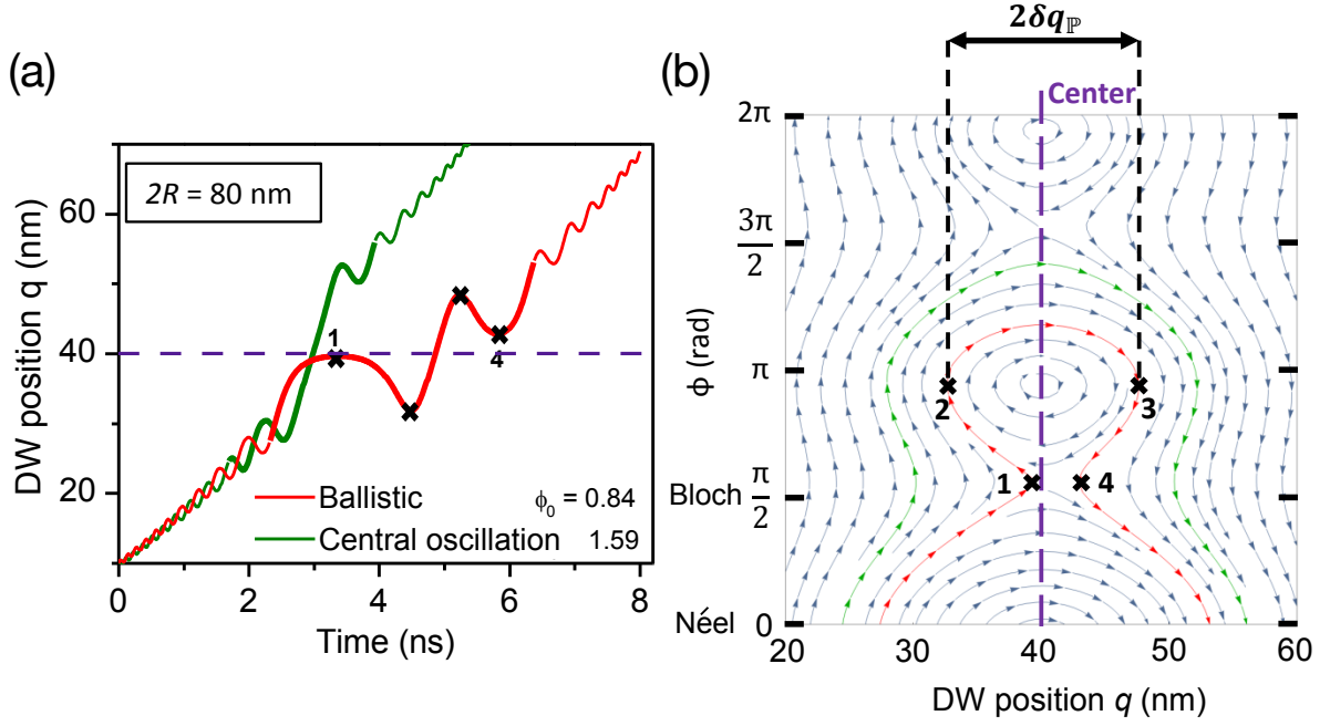
FIG. 10. Domain wall dynamics within a disc of 80 nm diameter under STT in the collective coordinate model with approximate effective fields. a) Time dependence of the position of the DW, for two different initial tilt angles being 48 deg. and 91 deg. and the same initial positions q_0 = 10 nm. b) Description of the possible trajectories of the DW in the space of the collective coordinates. \phi = 0 corresponds to a Néel DW and \phi = \pi/2 to a Bloch DW and the landscape is \pi periodic in the \phi direction. The colored trajectories correspond to the bold-colored parts of the trajectories of panel (a). The contour between the labels 1,2,3 and 4 of the red trajectory is very close to the retention pond frontier \partial\mathbb{P} .
