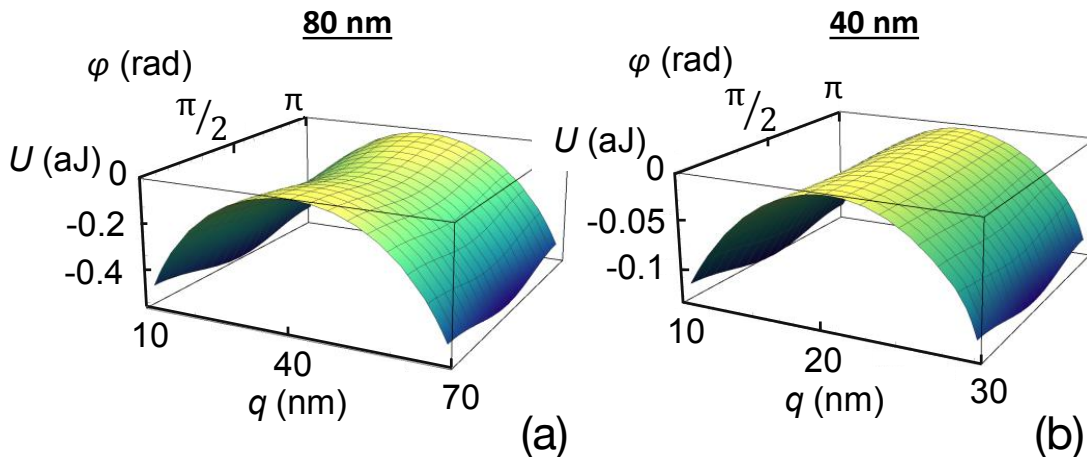
FIG. 5. Energy landscapes U_{\text{tot}} extracted from micromagnetic simulations for all positions q and tilt angles \phi for a straight domain wall in perpendicularly-magnetized discs of diameters (a): 80 nm and (b): 40 nm. A constant offset was added to the energy landscape to have the energy maximum be zero.
