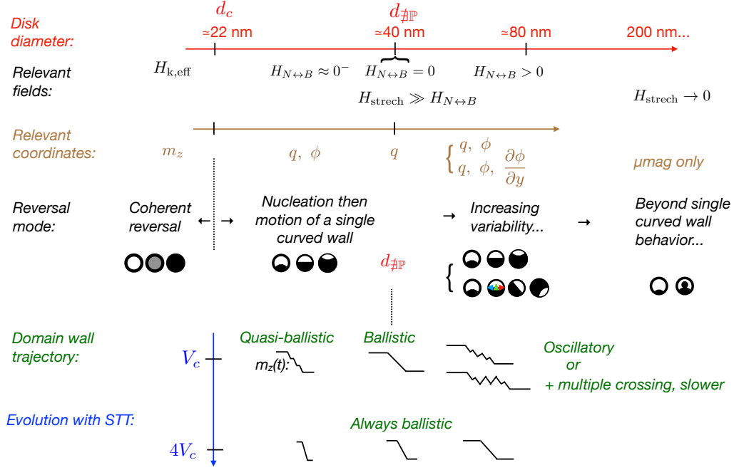
FIG. 11. Summarized description of the main features of the domain wall dynamics induced by spin-torque in perpendicularly magnetized discs. The disc diameter d_{\#P} is the one for which the position degree of freedom and the tilt degree of freedom of the domain wall get maximally independent when the wall crosses the disc center. The numerical values are for the material parameters of the theoretical sections. The conclusions of ref. [6] are also included.
