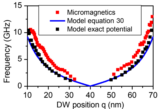
FIG. 9. Absolute value of the frequency of the oscillatory part of the domain wall motion in a disc of diameter 80 nm. Relation between the inverse of the wall oscillation period and the mean wall position during this period as predicted by micromagnetics (red symbols) and by the q - \phi - U_{tot} model (black symbols). The blue line is frequency inferred by analogy with the infinite stripe (Eq. 30). The frequencies change sign at the middle of the disc.
