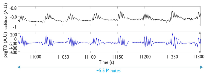
Figure 4. Comparison between the respiratory signals based on ccBioZ (Top) and TB from PSG (bottom) in a ~5.5 minute segment with multiple apneic episodes.
