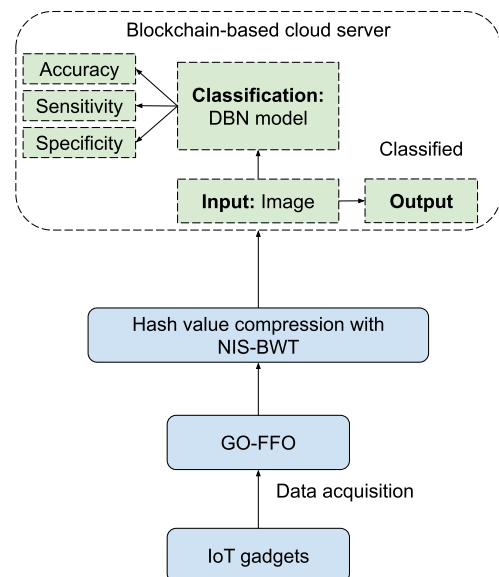
FIGURE 5. Architecture of the scheme proposed in [70].
