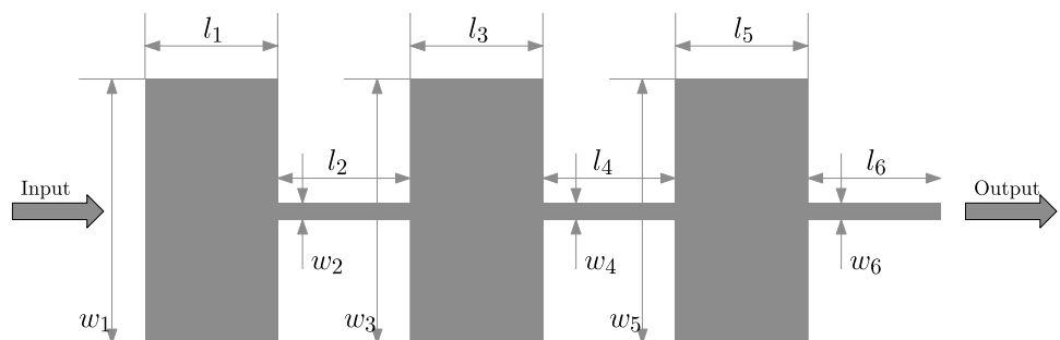
Fig. 4 Top-view of microstrip low-pass filter. We use 1 widths w_1 = w_3 = w_5 and 3 different lengths l_1, l_3, l_5 as design parameters
