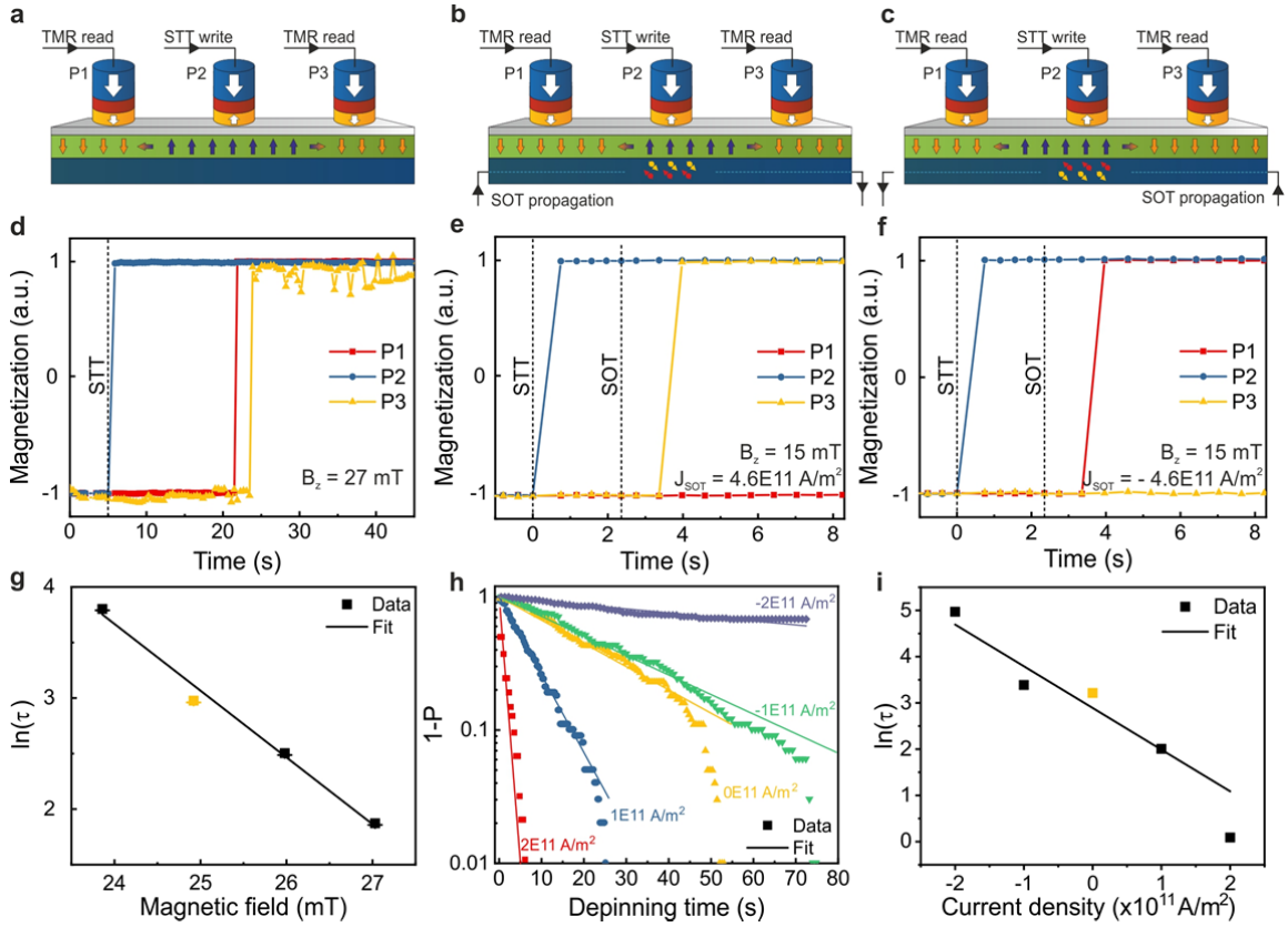
Fig. 4 | Full operation of a DW device with MTJs enabling STT write and TMR readout and SOT-driven DW transport. (a-c) Schematics explaining DW transport as observed in (d-f) respectively. (a,d) Field-driven domain expansion from P2 to both P1 and P3. (b, e) SOT-driven DW motion from P2 to P3 with positive current flow in the heavy metal and (c, f) SOT-driven transport from P2 to P1 with negative current. (g) Natural logarithm of the depinning time as function of external magnetic field. (h) Cumulative density functions (plotted as 1-CDF on logarithmic scale) of depinning time at a fixed field of 24.9 mT and varying current density obtained from 100 measurements at each current density and polarity. The data is fitted by an exponential law, resulting in the average depinning times as plotted in (i) as function of current.
