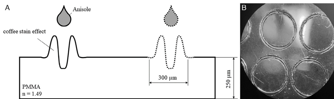
Figure 7. A) Schematic figure of inkjet-etched reservoir structure with double-sided walls; B) top view of etched reservoir structure on PMMA (microscope, d_{ring} = 4 mm). Reproduced with permission [25] Copyright 2018, SPIE Photonics Europe.
