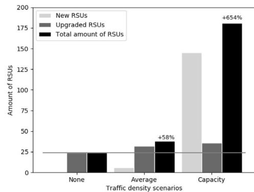
(b) Impact of traffic density correction on the amount of RSUs required for the pilot site
