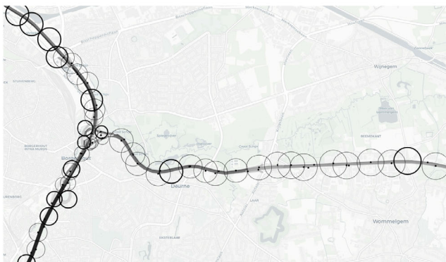
(a) Selected RSU locations within the pilot site, for average traffic density and the default range of 350 metre. Bold circles represent new RSUs, normal circles upgraded RSUs. Existing cabinets are shown by the black dots. The darker the highway segment, the higher the average traffic density on the segment
