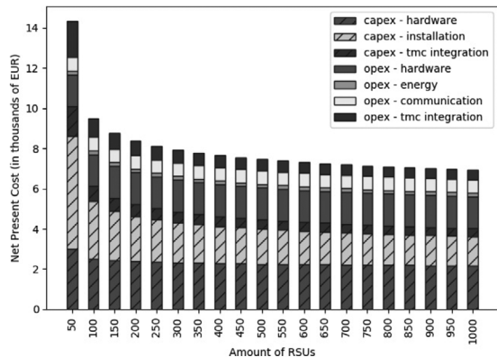
(a) Average Net Present Cost per RSU for different amounts of upgraded RSUs
