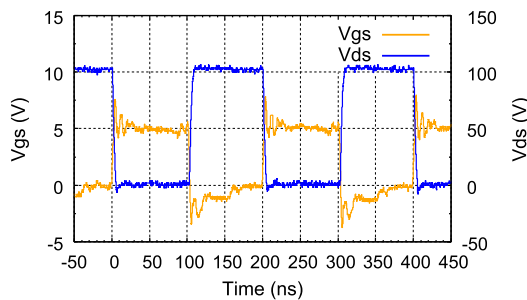
Fig. 14 5 MHz switching waveforms of the proposed GaN-IC at 100 V/4 A obtained by measurement.
