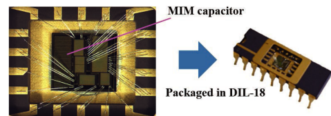
Fig. 10 Photomicrograph of GaN-IC packaged in DIL-18.
