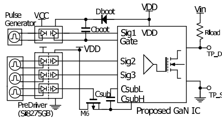
Fig. 11 Resistor-load type measurement circuit for GaN-IC.
