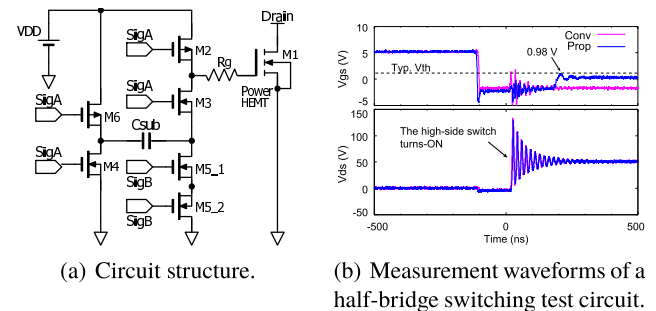
Fig. 1 Proposed 3-level gate driver [16].
