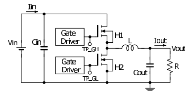
Fig. 16 Simplified schematic of SR buck-converter.
