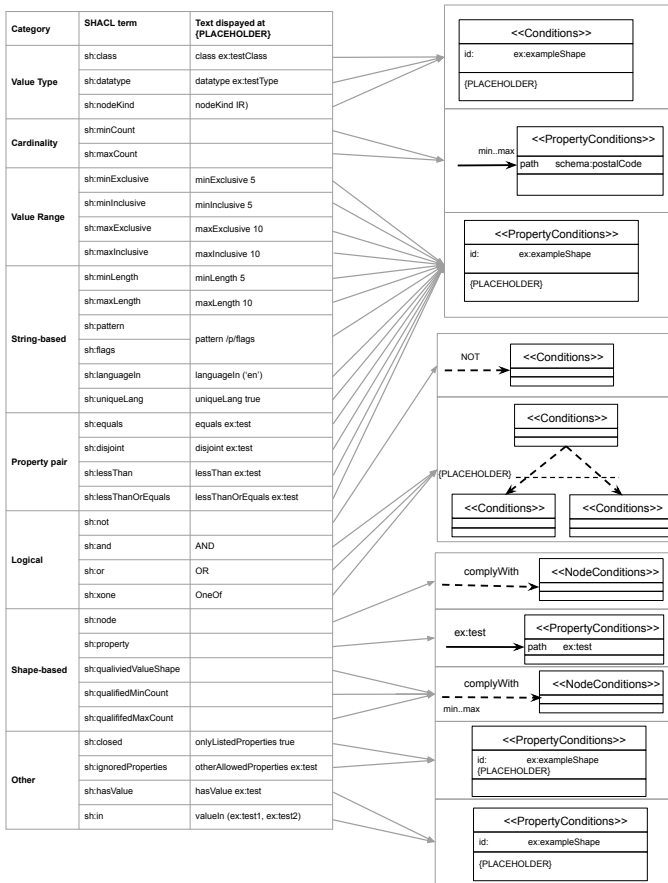
Figure 3.1: Correspondence between semantic constructs and ShapeUML : SHACL core constraints (left) and graphical notations (right).
