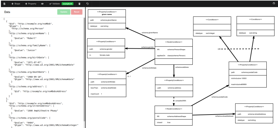
Figure 3.7: The user interface of our tool UnSHACled consisting of several panels supporting different editing approaches.
