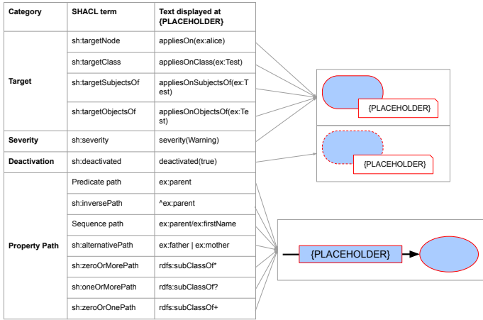
Figure 3.6: Correspondence between semantic constructs and ShapeVOWL : other relevant SHACL concepts besides core constraints (left) and graphical notations (right).
