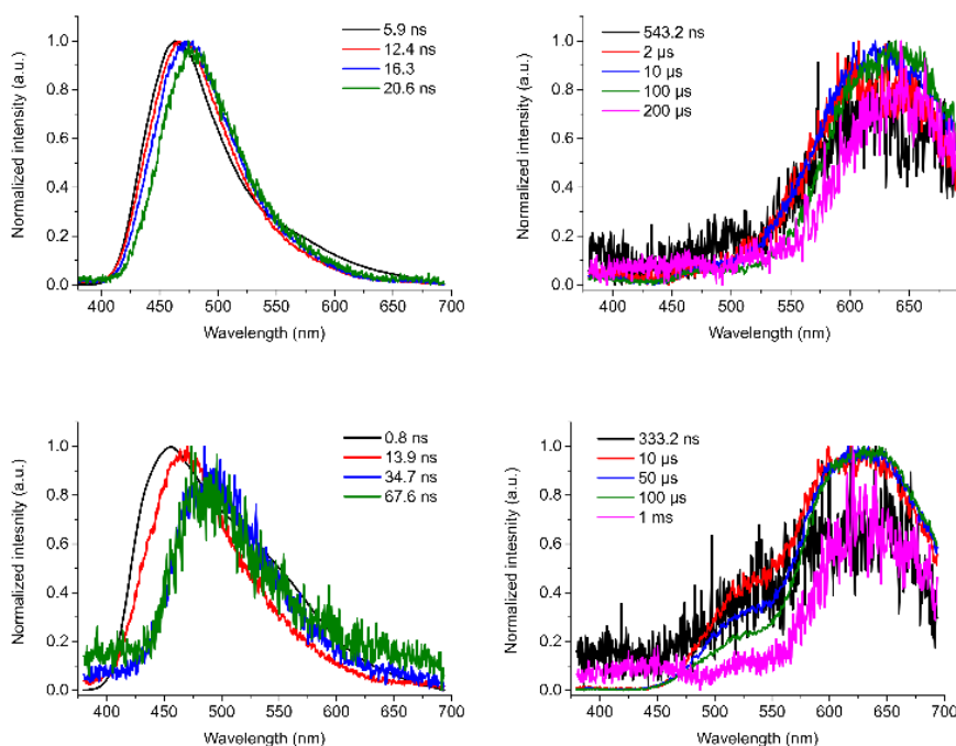
Figure 4. Snapshots of the emission at various time scales during prompt (left) and delayed emission (right) for BTaz-Th-PXZ at room temperature in chloroform (top) and in toluene (bottom) solution.
