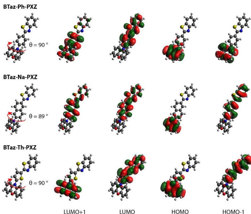
Figure 1. HOMO-LUMO spatial distributions for BTaz-Ph-PXZ , BTaz-Na-PXZ , and BTaz-Th-PXZ . Isocontour values of 0.02 (a.u.) were used for all orbitals.
