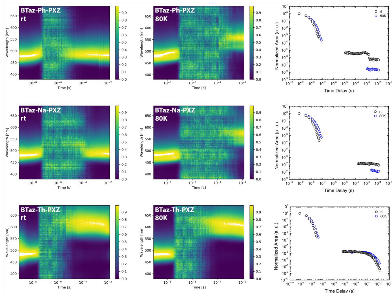
Figure 3. Normalised time-resolved emission spectra for BTaz-Ph-PXZ , BTaz-Na-PXZ , and BTaz-Th-PXZ in zeonex at room temperature (left) and at 80 K (middle), and decay of the total emission for the three dyads in zeonex at room temperature (rt) and at 80 K (right). The noise arising between the prompt and delayed emission is coming from the CCD camera. The discontinuity in the room temperature decay of BTaz-Ph-PXZ at around 10^{-3} s is due to alteration of the laser settings during the decay measurement. Data points without signal have been omitted from the decay, but are retained in the contour plots.
