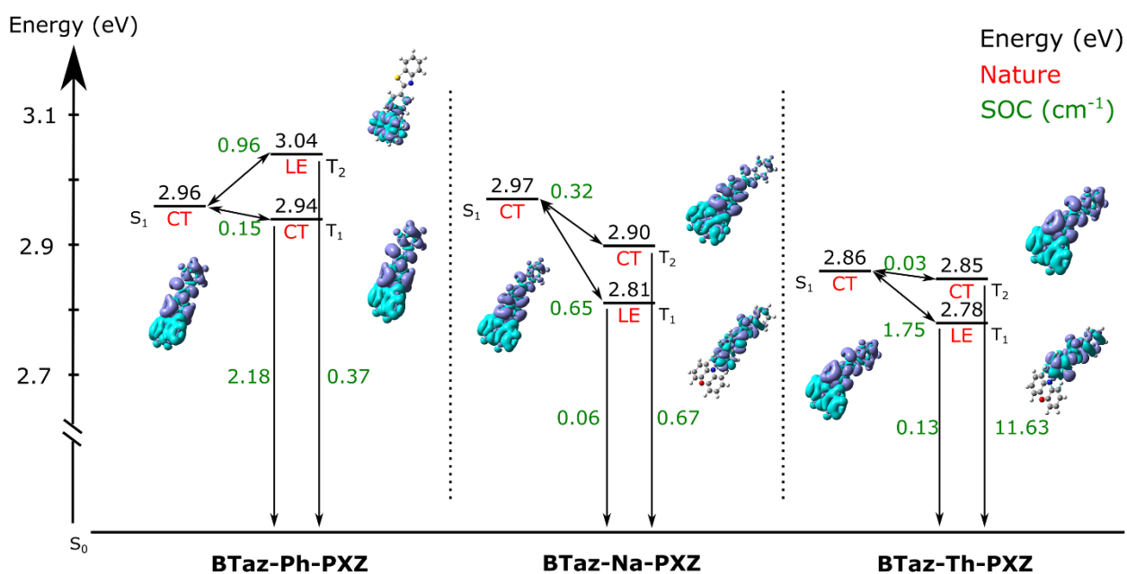
Figure 5. Schematic representation of the ground and excited state energy levels with their corresponding CT/LE character and the spin-orbit coupling values (in \text{cm}^{-1} ) between these various excited states as obtained using TDDFT calculations with LC-BLYP ( \omega = 0.17 \text{ bohr}^{-1} )/6-311G(d) under the TDA and applying the PCM (cyclohexane).
