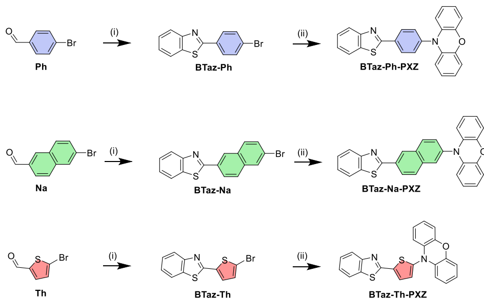
Scheme 1. Synthesis procedures for the three BTaz-Ar-PXZ emitters: (i) 2-aminothiophenol, sodium metabisulfite, DMF, reflux, 2 h; (ii) Pd(OAc) 2 , 10 H -phenoxazine, ( t -Bu) 3 P, Na t BuO, toluene, reflux, 16 h.
