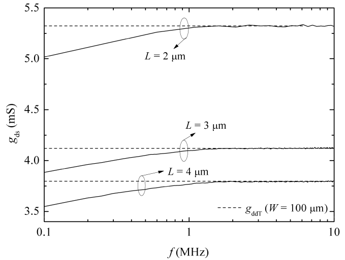
Fig. 4. Conductance frequency response at room temperature for GaN HEMTs with different gate lengths of 2–4 \mu\text{m} for V_g = 0 V and V_d = 5 V.
