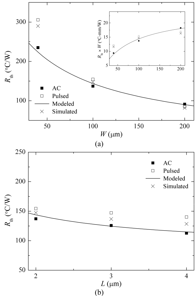
Fig. 6. Thermal resistance with (a) gate width for L = 2 \mu m and (b) channel length for W = 100 \mu m. AC/pulsed measured data are shown with closed/open squares. Simulated and modeled data are shown by crosses and lines, respectively. The inset in (a) analogously shows the dependence of the normalized thermal resistance as a function of the gate width.
