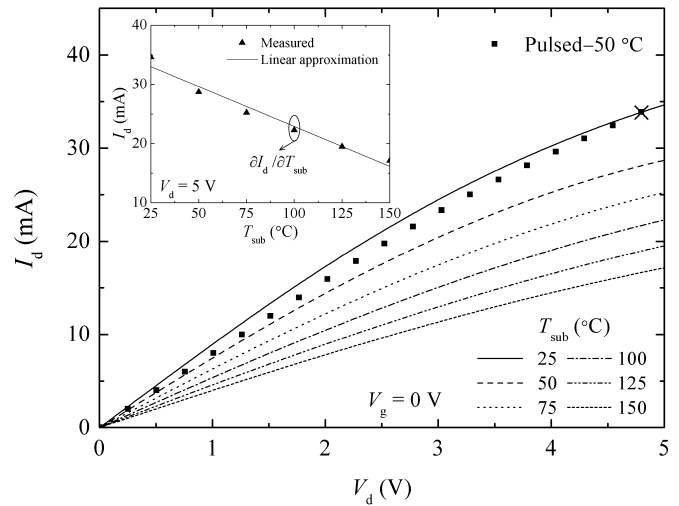
Fig. 3. Measured dc output characteristics (lines) at different substrate temperatures for the reference device and V_g = 0 V, and corresponding pulsed measurements at 50^\circ\text{C} (squares). Inset: resulting linear temperature dependence of the dc drain current for V_d = 5 V.
