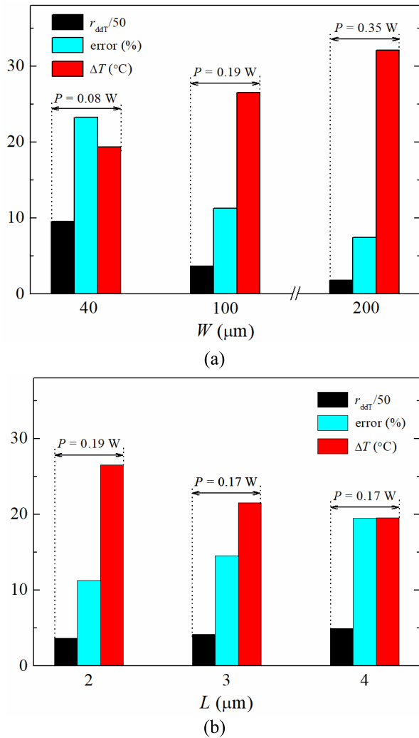
Fig. 7. Normalized ac output resistance without dynamic SHEs (black columns), relative error for the thermal resistance with both ac conductance and pulsed techniques (blue columns), and device temperature increment due to SHEs (red columns) with (a) gate width, for L = 2 \mu\text{m} and (b) channel length, for W = 100 \mu\text{m} .
