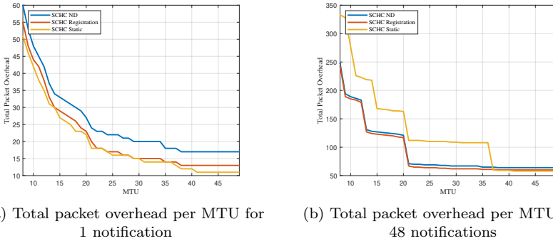
Figure 3.19: The total packet overhead for the complete LwM2M registration flow and different number of observation notifications.
