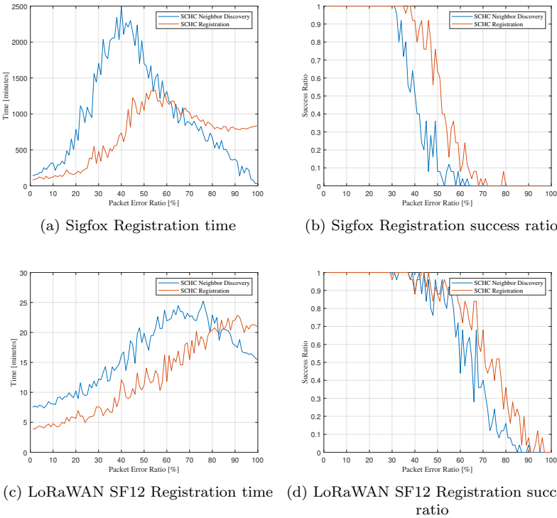
Figure 3.14: The total registration time for different packet error ratios (PERs) for both proposed mechanisms.
