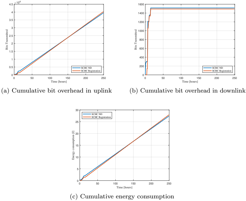
Figure 3.20: The cumulative bit and energy overhead for both solutions for a LoRaWAN SF12 device. Note that the SCHC ND mechanism will require less energy in uplink due to the double compression of the SCHC registration mechanism.
