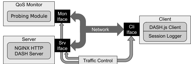
Fig. 4. Experimental environment
