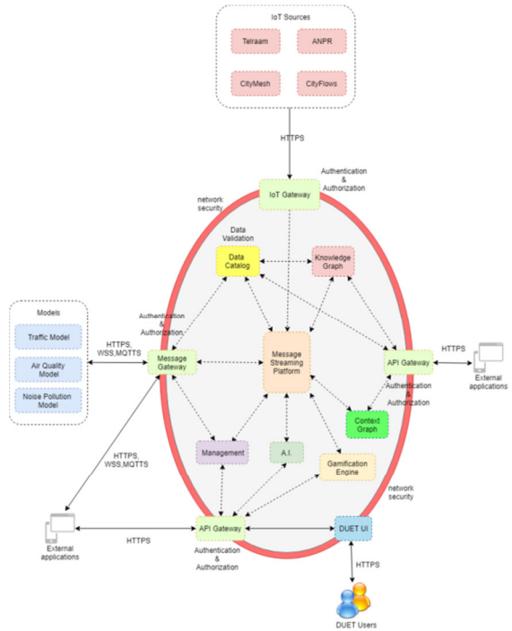
Figure 7. The security architecture of DUET’s digital twins platform.
