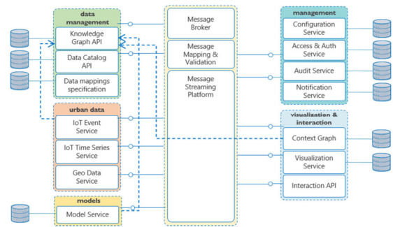
Figure 2. The T-Cell architecture comprises modules containing decoupled services that interact with each other through the central data broker.
