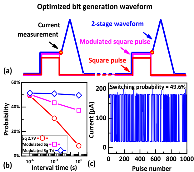
Fig.5. (a) The optimized 2-stage “square-triangular” waveform to remove the cumulative effect of failure-to-switch-on. Current is measured at the end of the square pulse. (b) Comparison of the switching probability measured with various interval time (○) using square pulse of 2.7 V, (□) modulated square pulse of 2.7 V, 2.8 V and 2.9 V for interval time of 1 \mu s, 1 ms and 1 s, respectively and (◇) 2-stage square-triangular pulse with square pulse amplitude being modulated in the same way as in (□). (c) Random bit stream generated with interval time= 1 s using the 2-stage square-triangular waveform with modulated square pulse amplitude (◇).
