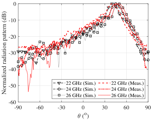
Fig. 4. Normalized simulated and measured radiation patterns in yz -plane at different frequencies.
