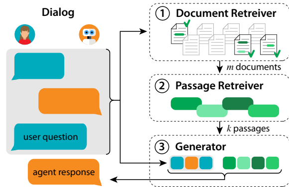
Figure 1: Our proposed pipeline dialog system.
