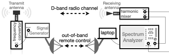
Fig. 1. Channel sounding architecture.
