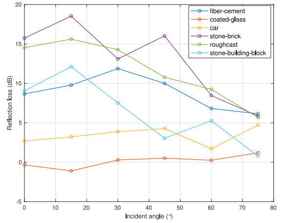
Fig. 6. Specular reflection loss as a function of incident angle for different surfaces for frequency 140 GHz.
