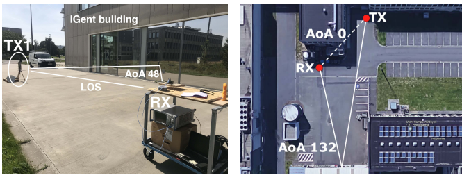
Fig. 5. Angular analysis based on environmental characteristics.
