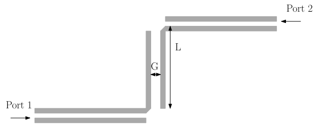
Fig. 4. Application I: Geometry of the microstrip bandpass filter (top layer).
