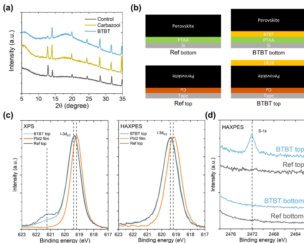
Fig. 4: (a) XRD measurements performed on lift-off samples with and without the interlayers. (b) Illustration of the four different configurations used for XPS and HAXPES measurements. (c) XPS and HAXPES measurements performed on lift-off samples concentrating on the I-3d 5/2 core level. (d) HAXPES measurement performed on all configurations concentrating on the S-1s core level.
