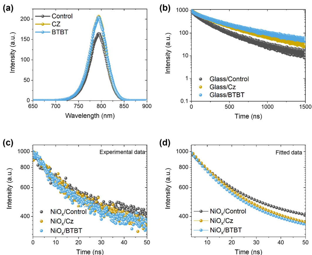
Fig. 2: (a) Steady-state PL and (b) time-resolved PL measurements for perovskite films on glass, with and without the interlayers. (c-d) Raw and fitted data of time-resolved PL measurements for perovskite films with and without interlayers on the HTL (NiO x ).
