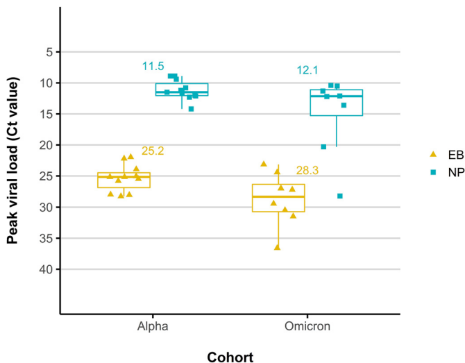
Figure 4. Comparing EB and NP peak viral loads between alpha and omicron cohorts, measured by qPCR ct values. This figure shows the peak viral loads expressed as qPCR ct values in both EB and NP in the immuno-naïve alpha-infected cohort (n = 11) and the partly boosted omicron-infected cohort (n = 8). Median peak viral loads are added. EB, exhaled breath; NP, nasopharyngeal.
