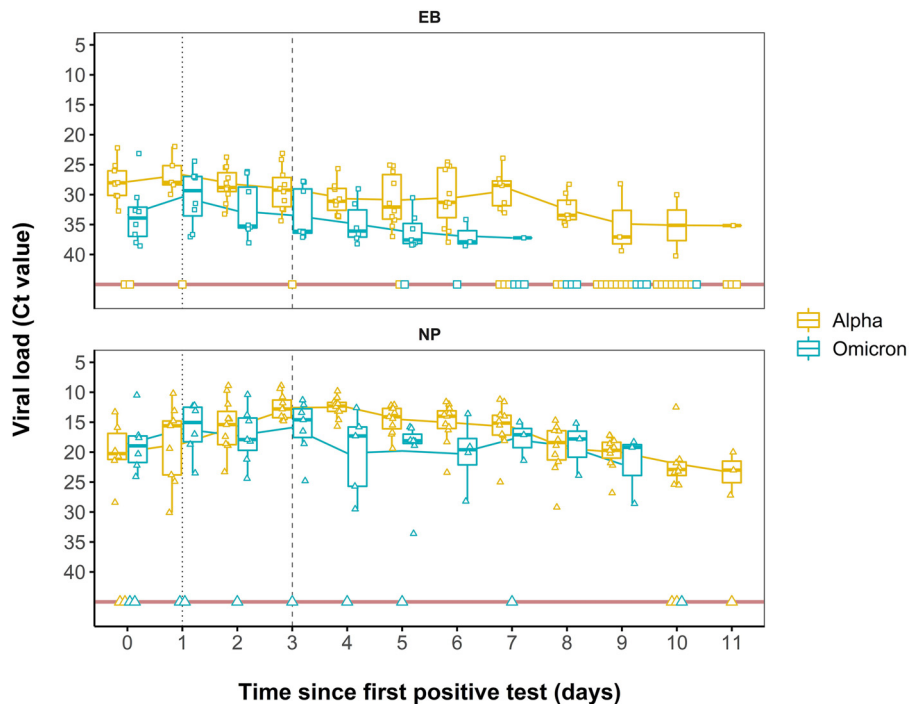
Figure 2. EB and NP shedding patterns, comparison between cohorts. The figure shows EB (top) and NP (bottom) qPCR ct values for the different cohorts (alpha vs. omicron patients). They are stratified by day since first positive test. The dotted line represents the day EB peaked, the dashed line the day the NP peaked. The horizontal red line represents negative tests. EB, exhaled breath; NP, nasopharyngeal.
