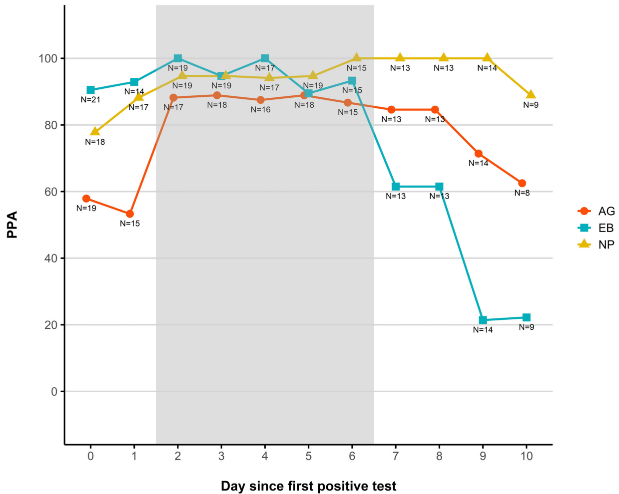
Figure 5. Comparing the positivity of EB qPCR to NP qPCR and NP RAT throughout infection. This figure shows the positivity of the different tests in comparison to aggregate positivity. Data from the alpha and omicron cohorts are combined and stratified by day of testing. The positivity of EB qPCR is equal to that of NP qPCR and superior than NP RAT on days 0-1 and 2-6 and inferior to other tests on the days after. Due to scarcity of data, days 11 and over were excluded. The number of observations is indicated below each point in the graph. EB, exhaled breath; NP, nasopharyngeal; NP RAT, NP rapid antigen testing.
