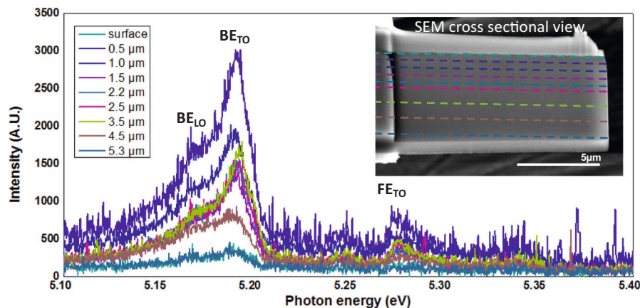
Fig. 3. CL spectra recorded at different positions on sample #D in cross section. Every position corresponds with a depth in the sample. These positions are marked by the same colours in the SEM micrograph of the inset.
