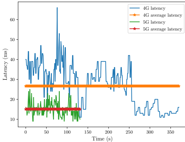
Fig. 4: Latency measurements.
