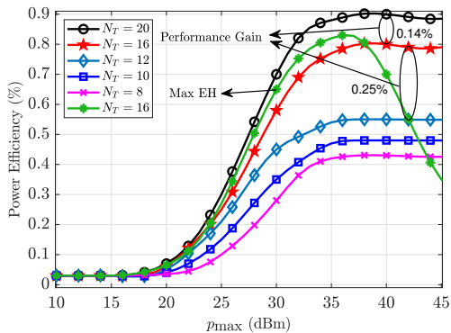
Fig. 2. Power efficiency versus maximum allowed transmit power.
