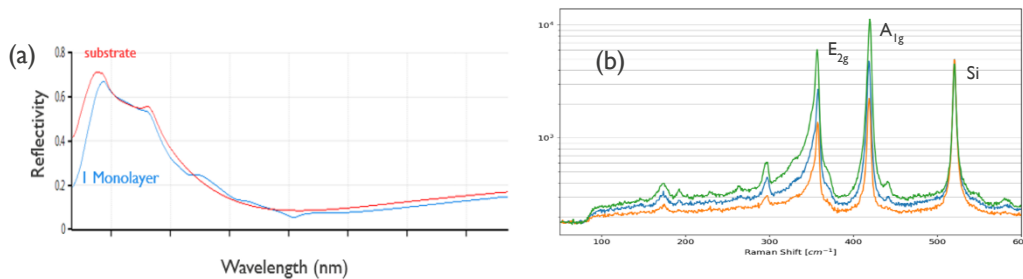
Figure 2: (a) Scatterometry spectrum for substrate (red) and one monolayer of \text{WS}_2 on substrate (Blue), (b) Raman spectrum for layer of \text{WS}_2 with different thicknesses.
