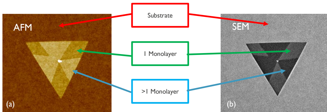
Figure 3: 4 \times 4 \mu\text{m}^2 image of an isolated island of WS 2 (a) from AFM, (b) from SEM
