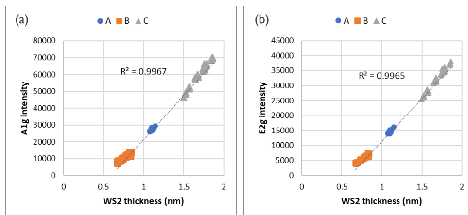
Figure 9: Correlation between WS_2 layer thickness obtain via scatterometry and the intensity of the peaks (a) A_{1g} and (b) E_{2g} from Raman Spectrum
