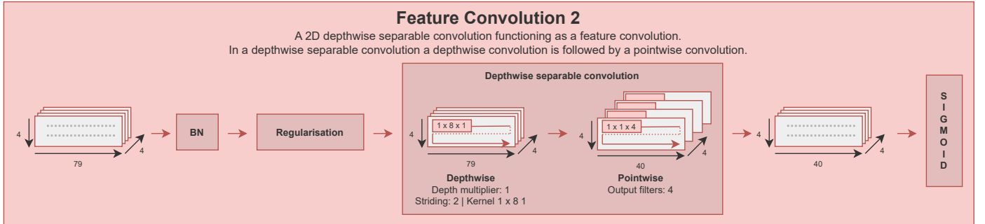
Figure 5: In-depth view of the second feature convolution within ECGencode, configured per ECGencode model 1 specified in Figure 1. The input is the output of the first feature convolution depicted in Figure 4. A depthwise separable convolution with a kernel of 1 \times 8 \times 1 and a stride of two is used. The pointwise convolution has a kernel of 1 \times 1 \times 4 and four output filters.
