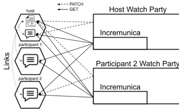
Fig. 4. An overview of the architecture for the watch party application.
