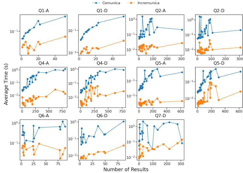
Fig. 2. Execution times for offline analysis, showing Incremunica outperforming reevaluation as query result size increases.
