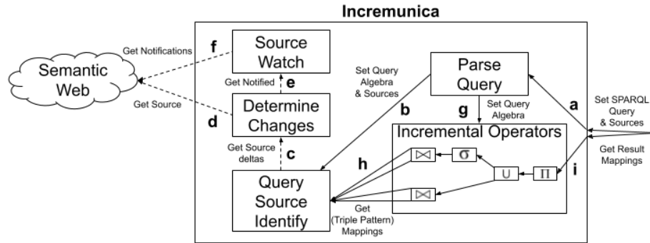
Fig. 1. High-level overview of the Incremunica architecture.
