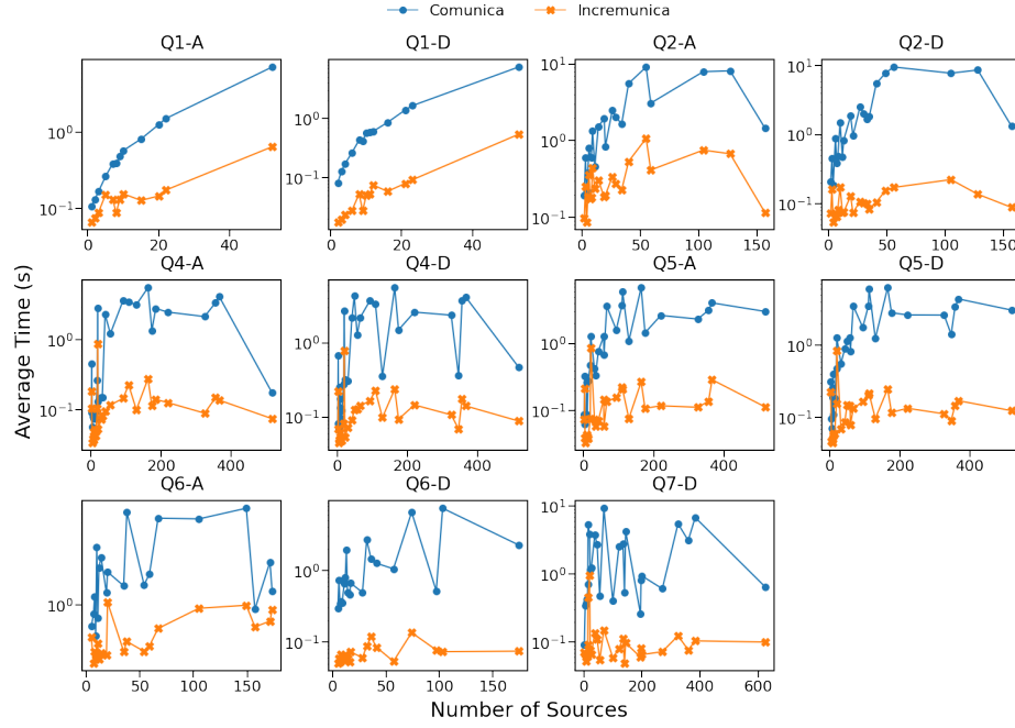
Fig. 3. Execution times for online analysis, highlighting Incremunica's advantage over reevaluation despite HTTP variability.
