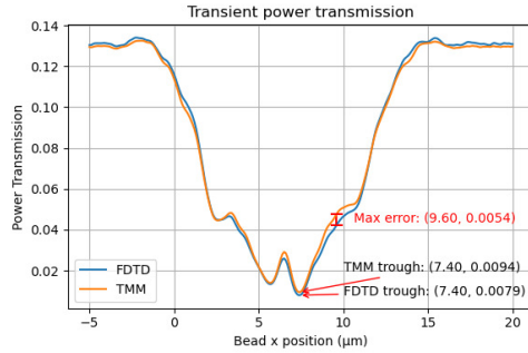
(a) Grating with 21 periods.
