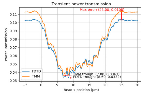
(b) Grating with 41 periods.
