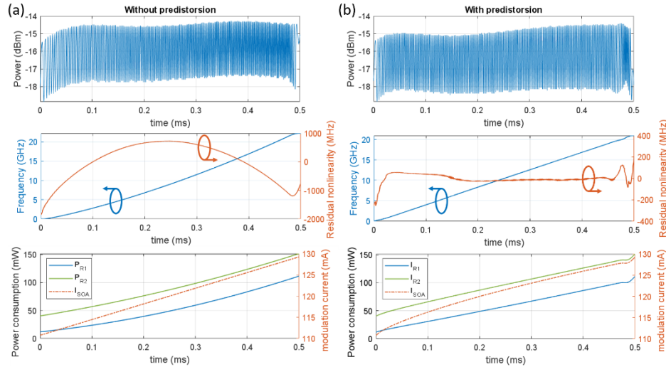
Fig. 8. Upper figures show the time traces obtained at the output of the unbalanced interferometer. Center figures show the laser frequency variation versus time (blue) with the corresponding residual nonlinearities (orange) before (a) and after (b) predistortion of the modulation signals. Bottom figures display the power consumption of the ring heaters (left axis) and the SOA driving current (right axis) during the frequency tuning.
