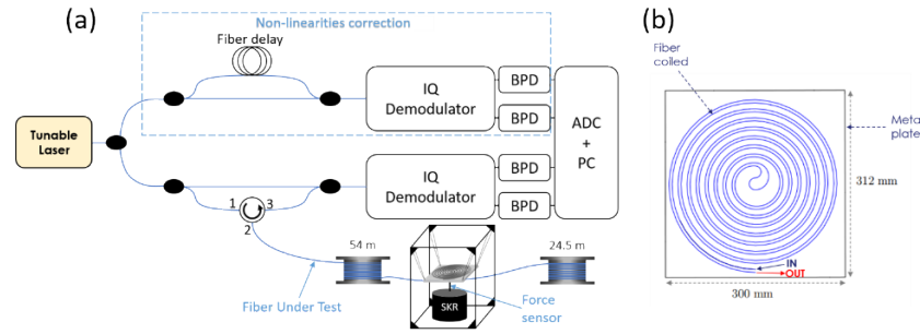
Fig. 9. (a) Schematic of the DOFS setup used, SKR: shaker. (b) Illustration of the fiber coiled on the metal plate.
