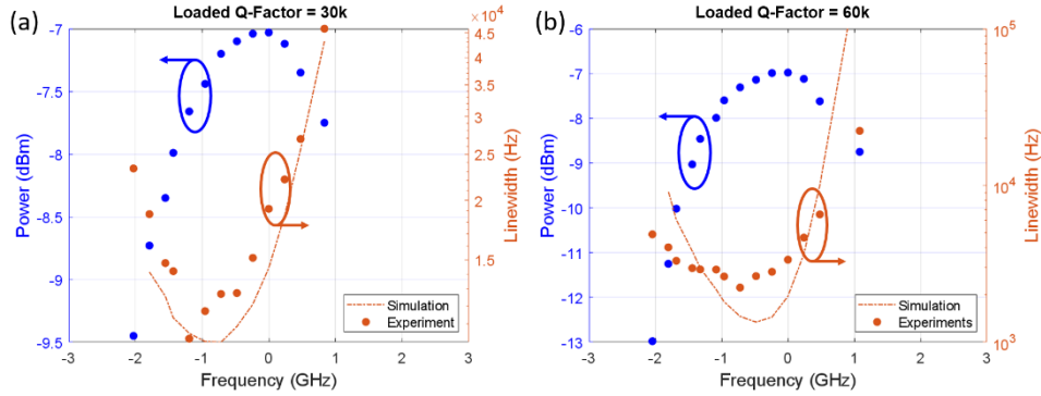
Fig. 6. Laser output power and the extracted linewidth from frequency noise measurement as a function of the detuned frequency for the two architectures studied (a) Q = 30,000 and (b) Q = 60,000 . The solid line shows the theoretical curve calculated from Eq. (4) with \alpha_H = 2.5 and the experimentally measured output power.
