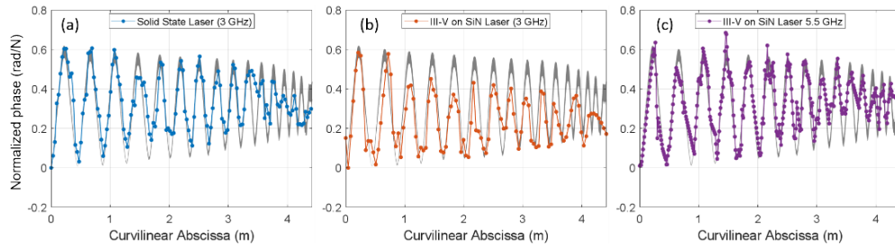
Fig. 10. Experimental DOFS measurements using different tunable laser sources. (a) Custom THALES RT solid state laser, (b) III-V-on-SiN laser with 3 GHz chirp amplitude, (c) high resolution measurement with III-V-on-SiN laser at 5.5 GHz chirp amplitude. The grey area shows the expected theoretical vibrational mode of the metal plate.
