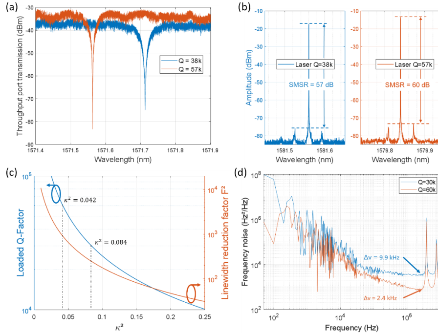
Fig. 5. (a) Transmission spectrum obtained on the through port of MRRs with a radius of 100 \mu\text{m} for a gap of 0.5 \mu\text{m} (blue) and 0.6 \mu\text{m} (orange). (b) Optical spectrum for the two different lasers studied. (c) Linewidth reduction factor F^2 and corresponding filter loaded Q-factor as a function of the rings coupling coefficient \kappa . Values for the limits \kappa=0.042 and \kappa=0.084 are indicated with arrows (loaded Q = 60,000 and 30,000 respectively). (d) Frequency noise spectrum for the two different lasers studied
