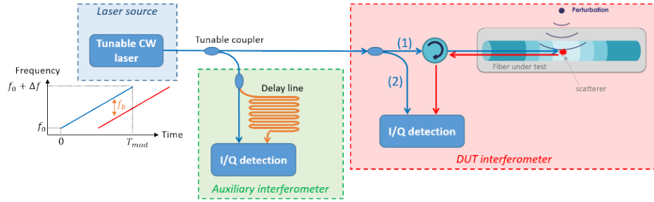
Fig. 1. OFDR interrogator schematic diagram.
