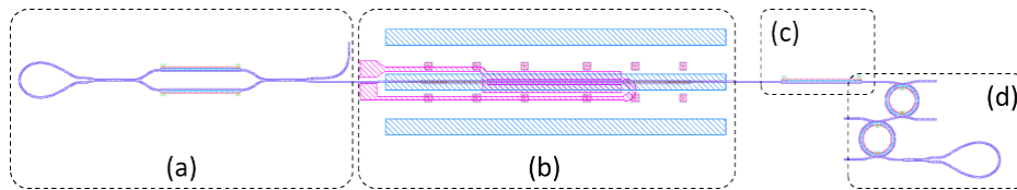
Fig. 2. Laser cavity design. (a) Front mirror, (b) gain medium, (c) phase section, (d) frequency selective back mirror.
