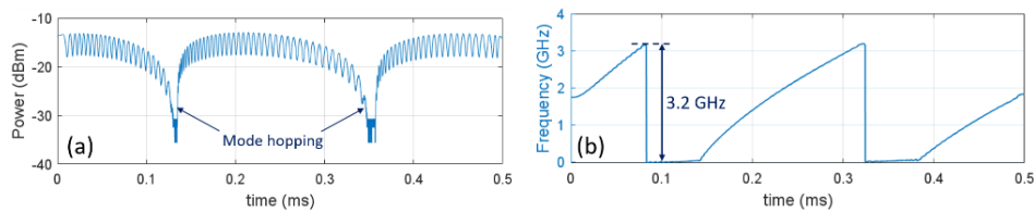
Fig. 7. (a) Time traces obtained at the output of the unbalanced interferometer. (b) Frequency vs. time curve with 500 MHz/mA modulation efficiency when only the gain section is modulated at a repetition rate of 1 kHz.
