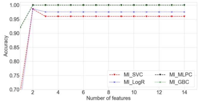
Fig. 8. Accuracy vs. number of features for G_{class_{SFN}} .
