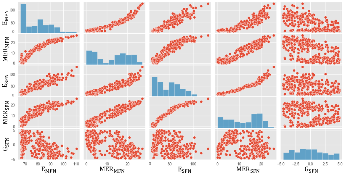
Fig. 4. Univariate distributions and pairwise relationship of E_{\text{MFN}} , \text{MER}_{\text{MFN}} , E_{\text{SFN}} , \text{MER}_{\text{SFN}} and G_{\text{SFN}} .
