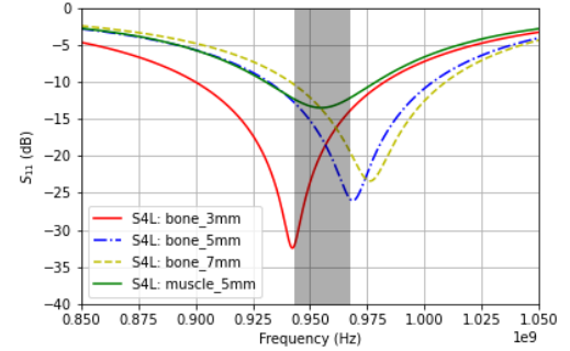
Fig. 5. |S_{11}| plot of the different leg tissues and filling epoxy thickness. The gray band denotes the aimed frequency band.
