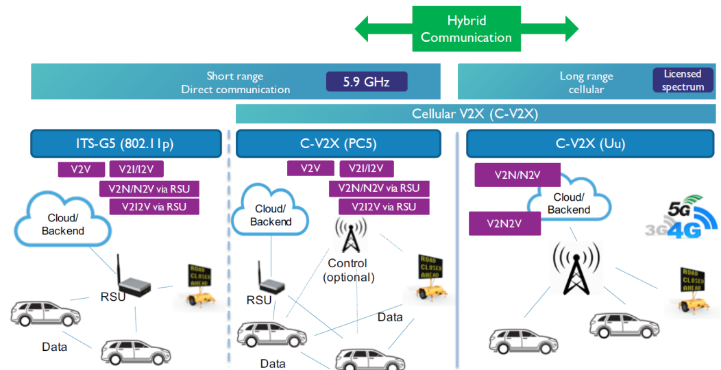
Figure 2. V2X technology classification [16].
