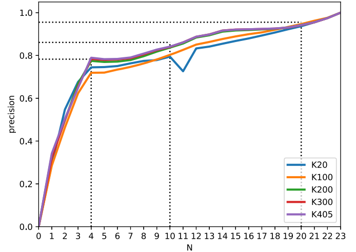
Fig. 3. Precision@N for different values of N obtained using our proposed approach with varying K values on validation sets. Each curve corresponds to the average obtained using the 10 \times 5 -fold cross validation.
