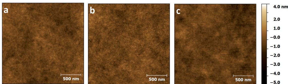
Fig. 4 AFM scans of the active layer blends (resulting in best solar cell performances) based on (a) \text{CPDT}(\text{FBTTh}_2)_2 , (b) \text{DTP}(\text{FBTTh}_2)_2 and (c) \text{TT}(\text{FBTTh}_2)_2 .
