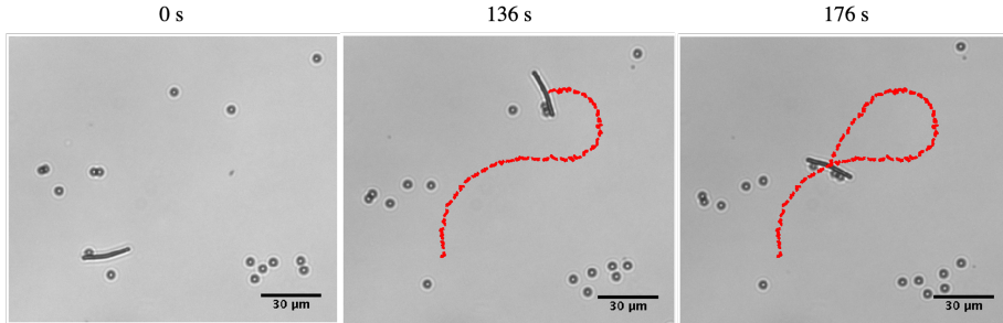
Figure 1: Sideways propelled Pt/Au rod collecting polystyrene cargo particles ( \sim 0.005 w/v%) in aqueous hydrogen peroxide (2.8 wt.%) solution, scale bar is 30 \mu\text{m} .
