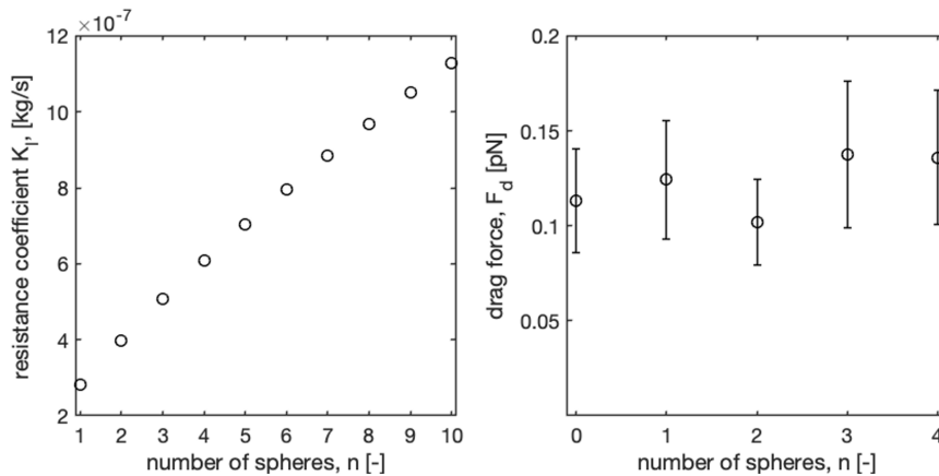
Figure 3: On the left: resistance coefficient K_l as a function of the number of spheres n attached to the sideways moving rod. On the right: drag force on a sideways propelled rod with n -attached spheres in aqueous hydrogen peroxide (2.8 wt.%) solution.
