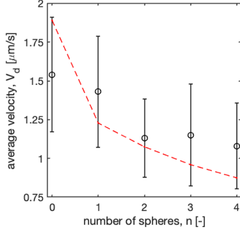
Figure 2: Velocities of a sideways propelled Janus rods of length \sim 20 \mu\text{m} that are pushing n polystyrene spheres in aqueous hydrogen peroxide (2.8 wt.%) solution (averaged for each loading over 3 different rods). The dashed red line represents the velocities calculated from eq. 1 with a resistance coefficient of the rod K_r calculated from eq. 2, and the resistance coefficient of n polystyrene spheres K_1 obtained from the beads model.
