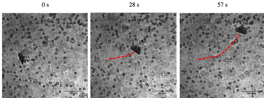
Figure 4: Sideways propelled Pt/Au rod collecting polystyrene cargo particles ( \sim 0.02 w/v%) in aqueous hydrogen peroxide (2.8 wt.%), scale bar is 30 \mu\text{m} .
