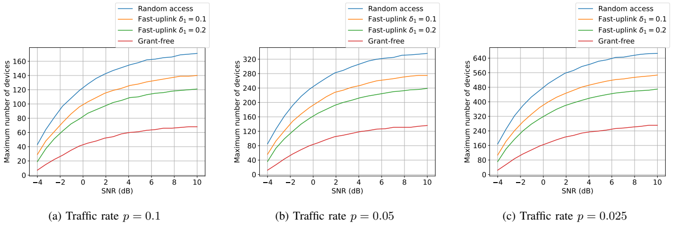
Fig. 5: Comparing the connection density of uplink access schemes where devices need to satisfy a maximum outage probability of 0.01
