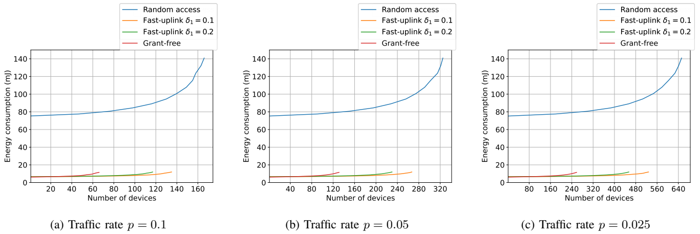
Fig. 6: Comparing the energy consumption of uplink access schemes where devices need to satisfy a maximum outage probability of 0.01
