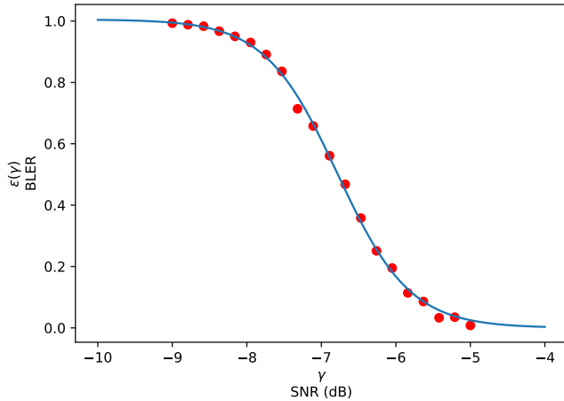
Fig. 4: Fitted BLER curve
