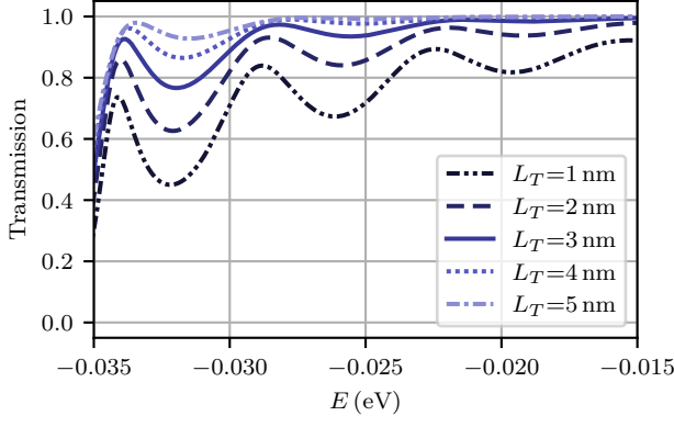
FIG. 7. Effect of the parameter L_T on the transmission through the nanoconstriction as a function of the energy E for the valley \mathbf{k}_D . The employed parameters are: V_0 = 0.45 eV, W_0 = 10 nm, W_1 = 4 nm, and L = 100 nm.
