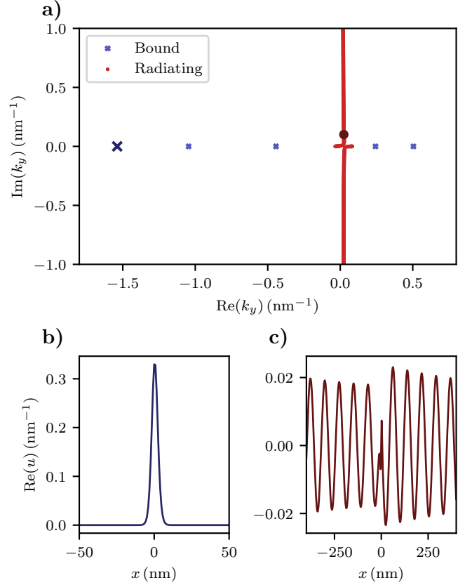
FIG. 2. (a) Eigenvalues of (3) distributed in the complex plane for valley \mathbf{k}_D . The hyperbolic secant potential (14), with V_0 = 0.45 eV and constant W = 10 nm, was chosen together with an energy E equal to -0.02 eV. (b) Plot of the real part of u as a function of the position x for the bound eigenmode associated with k_y = -1.54 \text{ nm}^{-1} (indicated by a large blue cross in (a)). (c) Plot of the real part of u as a function of the position x for the radiating eigenmode associated with k_y = (0.023 + 0.096i) \text{ nm}^{-1} (indicated by a large red dot in (a)).
