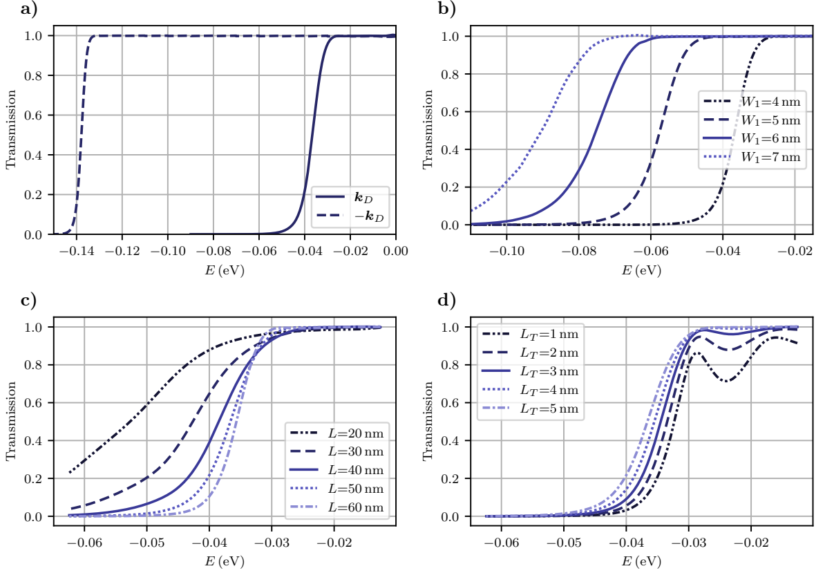
FIG. 6. Transmission through the nanoconstriction as a function of the energy E for various design parameters. The transmission for the valleys \mathbf{k}_D and -\mathbf{k}_D is depicted in (a) for V_0 = 0.45 eV, W_0 = 10 nm, W_1 = 4 nm, L = 50 nm, and L_T = 5 nm. The effect of the width of the narrow section W_1 , the length of the narrow section L , and the length of the transition region are illustrated by (b), (c), and (d), respectively. In (b)-(d) the same parameters as in (a) are employed except for the one that is varied. Only valley \mathbf{k}_D is considered in (b)-(d).
