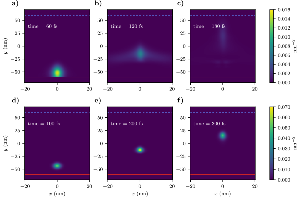
FIG. 5. (a)-(f) Snapshots of the probability density, demonstrating the valley filtering effect of a nanoconstriction. Plots (a)-(c) are attributed to valley \mathbf{k}_D and (d)-(f) to -\mathbf{k}_D . The potential profile corresponds to (14) with V_0 = 0.45 eV and with W varying with the position y according to (15). The full width at half maximum of the broad part of the potential W_0 is 10 nm, while the full width at half maximum of the narrow section W_1 equals 4 nm. The length of the narrow section L is 50 nm and the length of the transition region is characterized by L_T = 5 nm. The spectral content of the incoming mode is centered around E = -0.06 eV.
