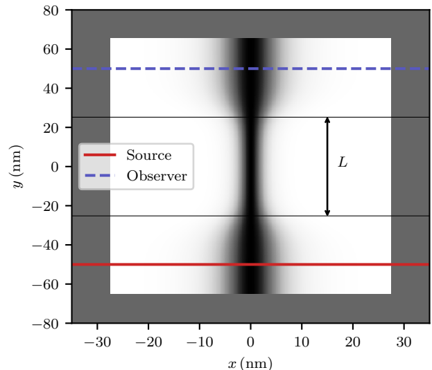
FIG. 3. Illustration of the simulation setup of an electrostatic waveguide with nanoconstriction. The middle region (black) represents a two-dimensional plot of the potential profile. The simulation domain is terminated by an absorbing layer (grey region). The constriction is of length L . The source is indicated by a red line, while the blue, dashed line represents the observer.
