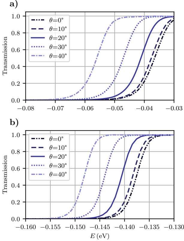
FIG. 9. Effect of the parameter \theta , the angle between the axis of the waveguide and the tilting direction, on the transmission through the nanoconstriction as a function of the energy E for valley \mathbf{k}_D (a) and valley -\mathbf{k}_D (b). The employed parameters are: V_0 = 0.45 eV, W_0 = 10 nm, W_1 = 4 nm, and L = 50 nm.
