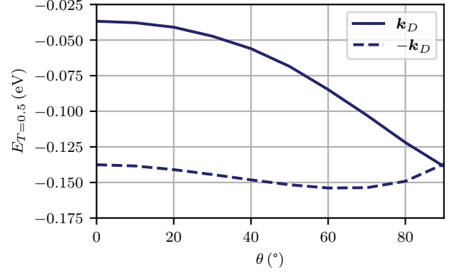
FIG. 10. Energy value E_{T=0.5} for which the transmission function equals 0.5 as a function of the mismatch angle \theta for both valleys \mathbf{k}_D and -\mathbf{k}_D . The employed parameters are: V_0 = 0.45 eV, W_0 = 10 nm, W_1 = 4 nm, and L = 50 nm.
