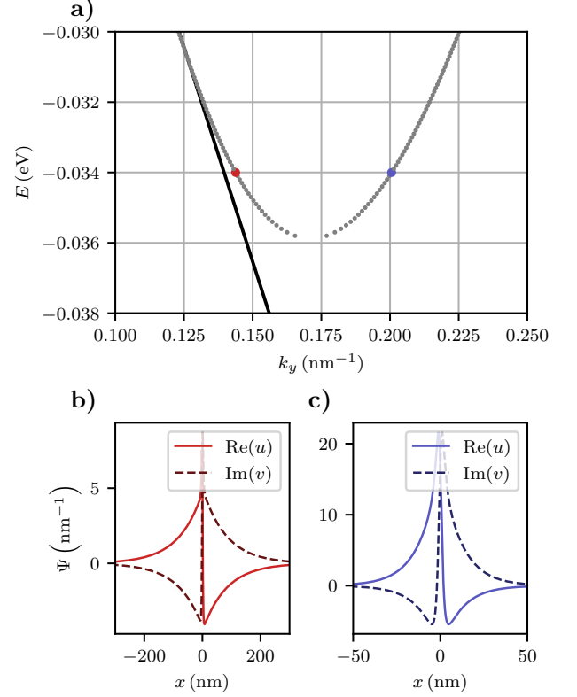
FIG. 8. (a) Detail of the dispersion relation of the lowest-order forward-propagating bound mode in a hyperbolic secant potential (14), with parameters W = 4 nm and V_0 = 0.45 eV. The eigenvalues k_y were calculated by means of the numerical procedure outlined in Section III. The considered valley is \mathbf{k}_D . The two eigenmodes indicated with a red and blue dot correspond to an energy E of -0.034 eV. They are plotted as a function of the position x in (b) and (c), respectively. (b) corresponds to k_y = 0.142 nm ^{-1} , while k_y is equal to 0.200 nm ^{-1} for the eigenmode presented in (c).
