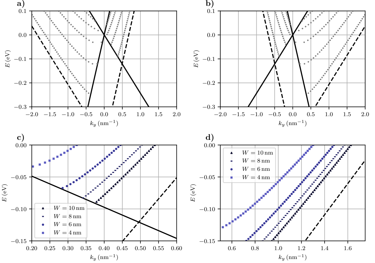
FIG. 4. (a)-(b) Plots of the eigenvalues k_y of the bound modes versus energy E for the hyperbolic secant potential (14) with W = 10 nm and V_0 = 0.45 eV. (a) Grey dots represent the eigenvalues corresponding to valley \mathbf{k}_D , while in (b) the eigenvalues associated with valley -\mathbf{k}_D are displayed. (c)-(d) Plots of the eigenvalue k_y of the lowest-order, forward-propagating bound mode as a function of energy E for a set of values of the full width at half maximum W for the valleys \mathbf{k}_D and -\mathbf{k}_D , respectively. For (a)-(d) the dispersion relation in the case of zero potential is given by the full, black line. The dashed black line is the dispersion relation in the case of a constant potential -V_0 . The eigenvalues k_y were calculated by means of the numerical procedure outlined in Section III.
