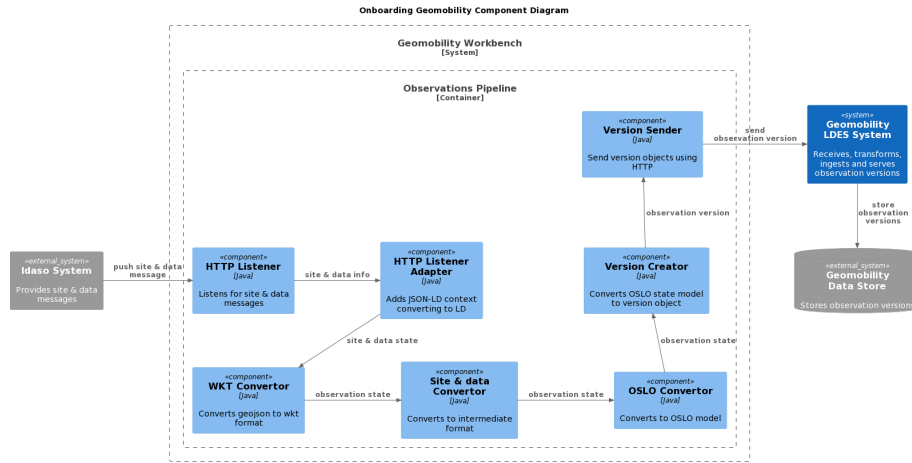
Fig. 3: Final pipeline for Geomobility to publish their datasets as an LDES
