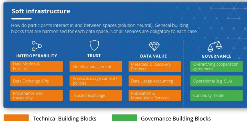
Fig. 1: Data Space building blocks to be implemented by the Data Space initiatives (source: Design Principles for Data Spaces position paper [8])
