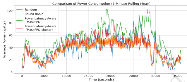
Figure 7: The average power trend on a real cluster
