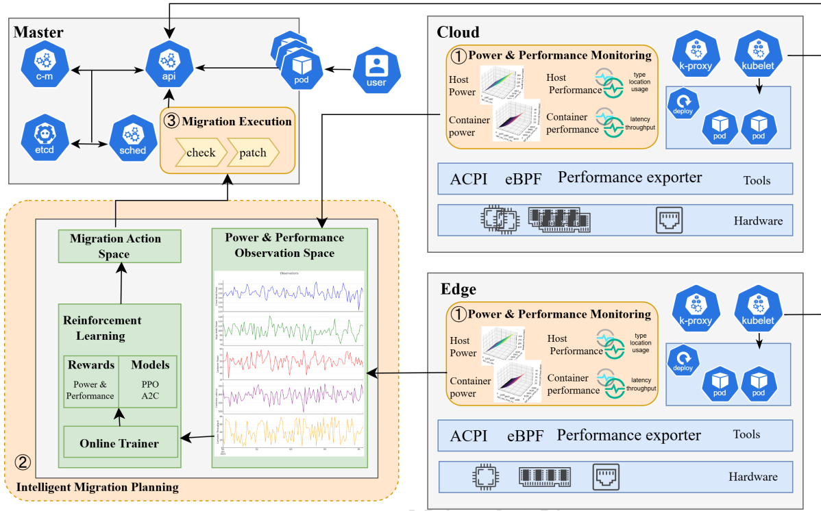
Figure 2: GreenWise: Kubernetes-based Computing Continuum Platform for Intelligent Migrating ML Services.
