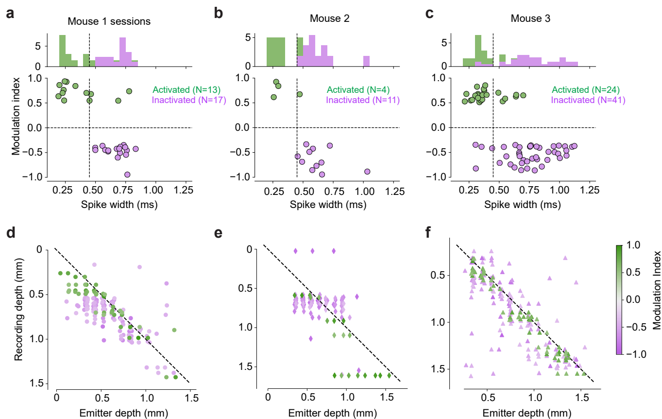
Extended Data Fig. 7 | Activation of putative inhibitory neurons in individual mice. a-c. Same data as in Fig. 4e, broken down by mouse, showing modulation index ( (R_i - R_0)/(R_i + R_0) ) (ordinate) as a function of trough-to-peak spike width of average waveforms. d-f. Same data as in Fig. 4g, broken down by mouse. Each
