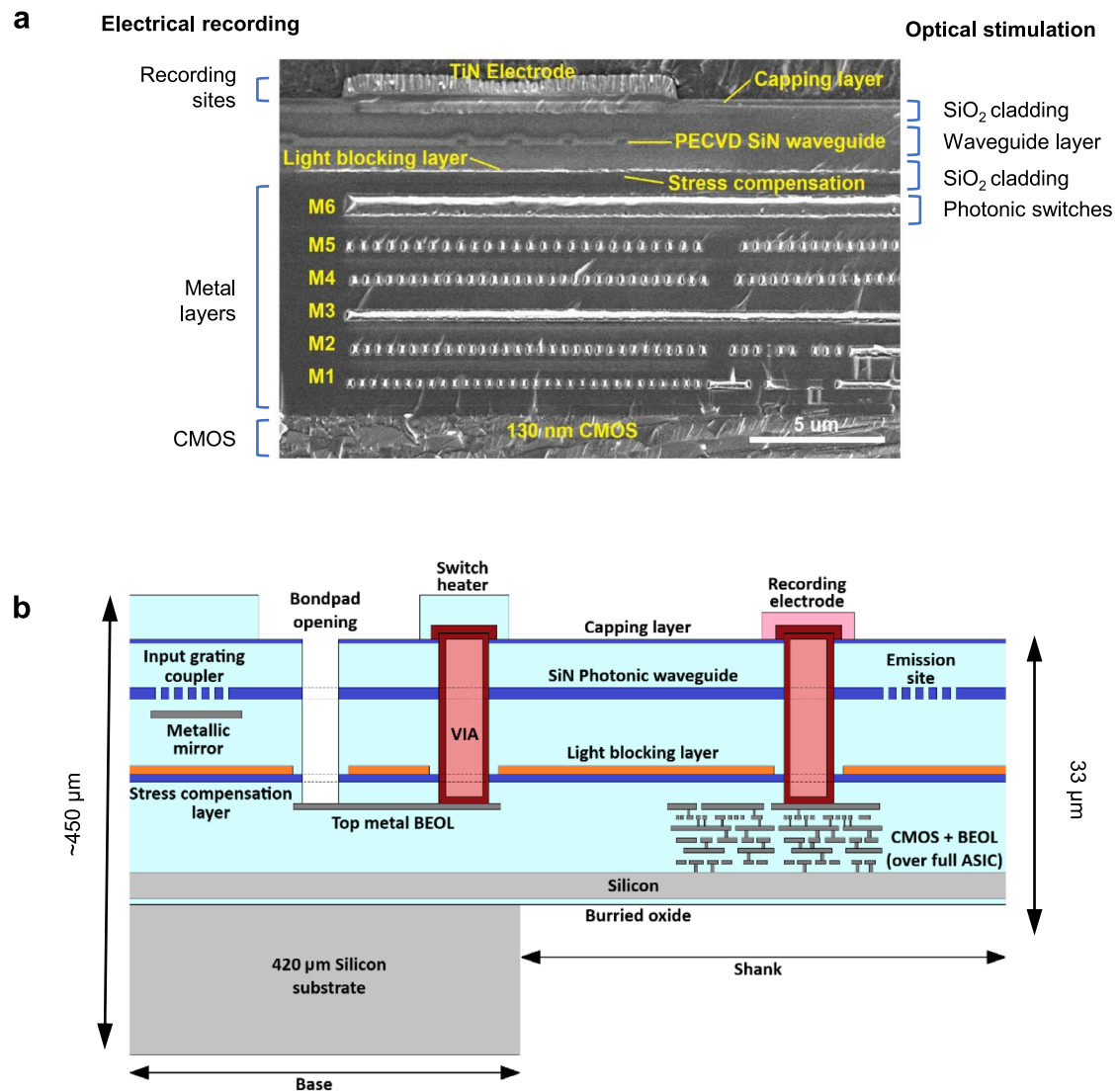
Extended Data Fig. 1 | The integrated CMOS/Photonics platform. a. Cross-section of the probe shank obtained with a scanning electron microscope (SEM) showing the monolithically integrated platform combining the CMOS platform (for electrical recording) and Si x N y -based photonics (for optical stimulation). Left labels: layers used for the recording sites and readout IC, based on the 130-nm SOI CMOS Aluminum back-end-of-line process (Al BEOL) that was developed for the Neuropixels 1.0 probe. They point to the 130-nm CMOS layer ( bottom ), the 6 Aluminum metal layers ( middle ) and the Titanium nitride electrode ( top ). Right labels: the photonic modules that were added between the M6 metal layer of the CMOS BEOL and the recording electrode to enable optical stimulation. The photonics also use the M6 metal layer for controlling the
