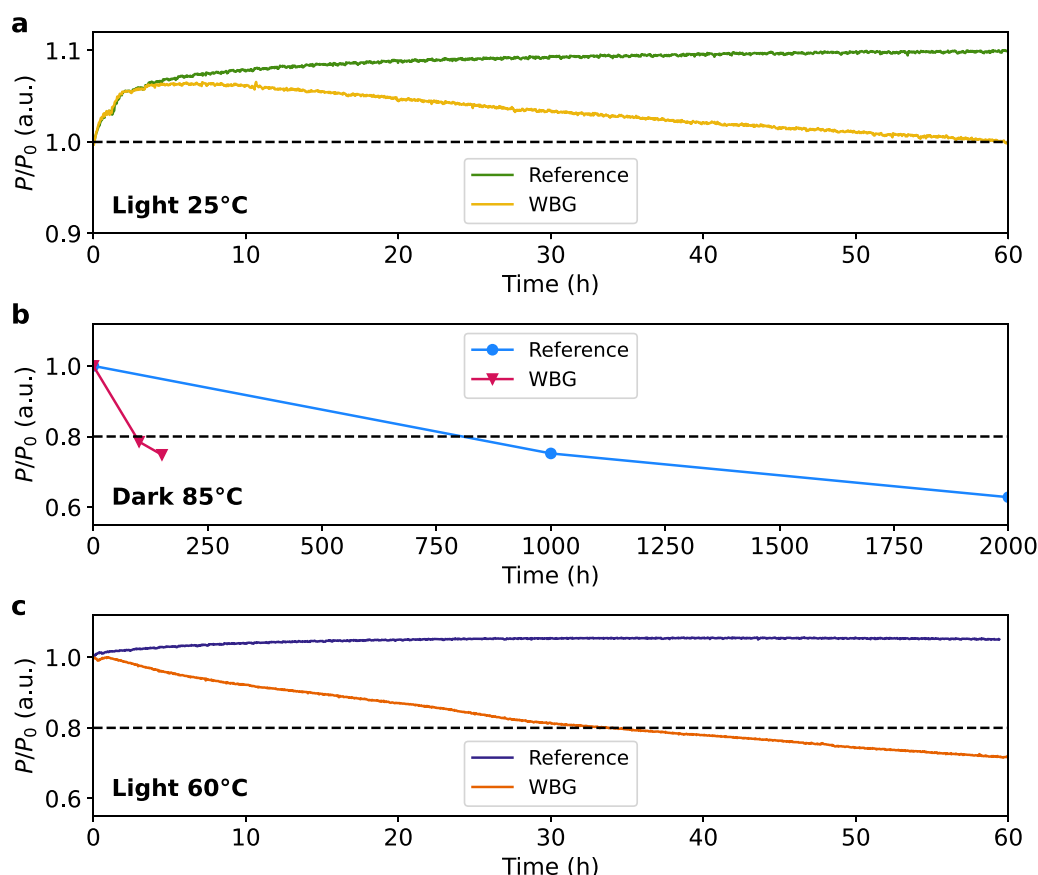
Figure 1. Performance evolution of the reference vs wide bandgap (WBG) samples under different stressing conditions: (a) ISOS-L1: maximum power point tracking (MPPT) under 1 Sun illumination at 25 °C, (b) ISOS-D2: dark storage at 85 °C and (c) ISOS-L2: MPPT under 1 Sun illumination at 60 °C. All tests were performed in a N_2 environment.
