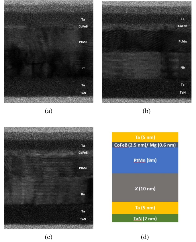
Figure 2. Cross-section TEM micrographs of the multilayers with (a) Pt, (b) Nb and (c) Ru seed layers annealed at 425 °C.
