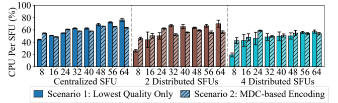
Figure 7: Average CPU usage across all cores, with 95% confidence intervals, for user counts of 8 to 64.
