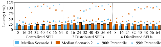
Figure 5: Median latency is stable for user counts of 8 to 64. Peak latencies, represented by the percentiles, increase more with the 90th percentile being stable.
