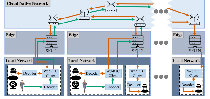
Figure 1: Proposed distributed SFU architecture for many-to-many volumetric streaming, supporting content forwarding between multiple SFUs. Each client can either serve as a sender, receiver or both.
