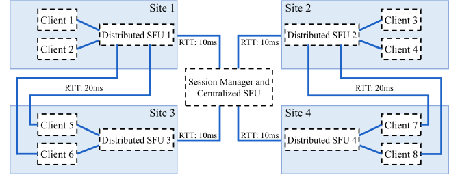
Figure 2: Bare-metal setup used for experimentation. Each SFU node can either serve as a normal SFU or as a simple switch node and each client node can host one or more WebRTC client applications.
