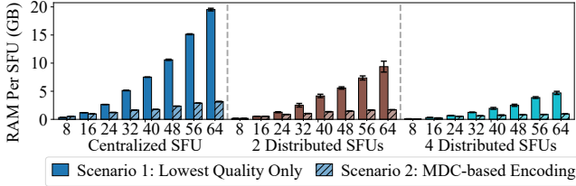
Figure 6: RAM usage per SFU, with 95% confidence intervals, for user counts of 8 to 64.
