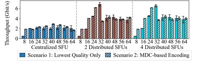
Figure 3: Total throughput of client data, with 95% confidence intervals, for user counts of 8 to 64.
