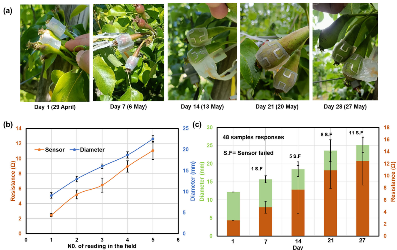
FIGURE 7 | Field deployment of stretchable sensors for real-time fruit growth monitoring. (a) Sequential images of the sensor integration on pear fruitlets over a 28-day growth period. (b) Correlation between the resistance change of four representative sensors and the corresponding fruit diameter measured with a vernier caliper. (c) The statistical summary of 48 deployed sensors highlights both functional devices and sensor failures due to connector detachment or environmental degradation during stretching.
