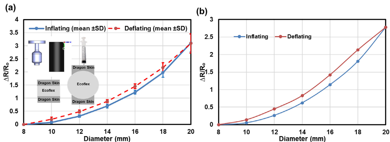
FIGURE 6 | Sensor characterization on soft balloon-shaped actuator to mimic the fruit growth (a) Averages across multiple sensors trials ( n = 7 , mean \pm SD), confirming reproducibility and reduced variability in the hybrid structure, with inset shows the design and fabrication of soft hybrid actuator using Ecoflex and Dragon Skin (b) Sensor hysteresis analysis between inflation and deflation cycles.
