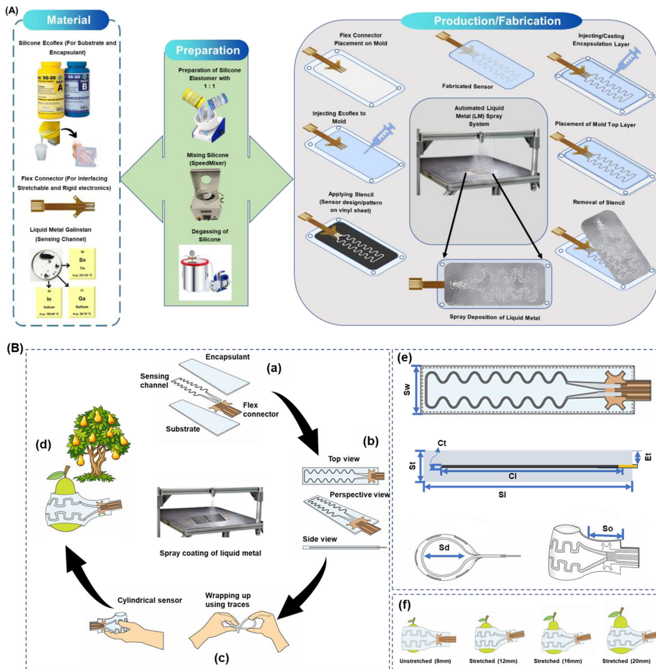
FIGURE 1 | (A) Fabrication workflow of the stretchable LM based strain sensor, illustrating material selection, silicone preparation, stencil assisted LM spray deposition, and final encapsulation. (B) Schematic representation of the sensor: Design, structural layout, and deployment concept of the stretchable sensor for fruit growth monitoring. (a) Layer-by-layer architecture showing substrate, sensing channel, encapsulant, and the flex connector. (b) Sensor geometry from different orientations (top, side, and perspective views). (c) Convert the planar sensor into a cylindrical configuration and a wrapping strategy for attachment. (d) Practical illustration of the sensor integration on fruit for monitoring diameter expansion during growth. (e) Dimensional analysis of the sensor, highlighting the dimensional overview of the planar and cylindrical sensors. (f) Conceptual demonstration of continuous fruit growth monitoring enabled by a sensor over developmental stages.
