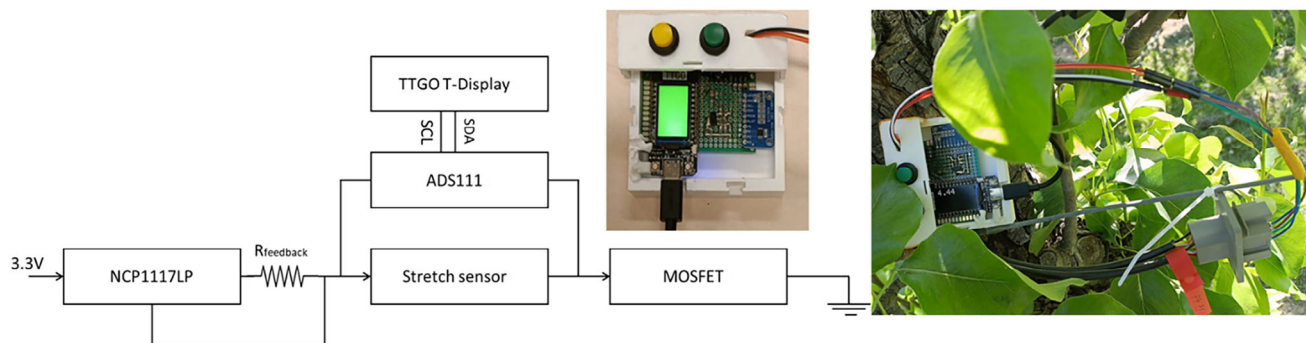
FIGURE 2 | Readout electronics for resistance measurement showing its block diagram and visuals of the manual portable measurement readout system.
