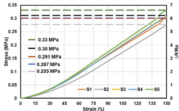
FIGURE 4 | Mechanical stability, resistance-strain, and stress-strain behavior of five sensors. Low stress range (0.255–0.33 MPa) demonstrates sensor compliance, ensuring negligible resistance against fruit growth forces.
