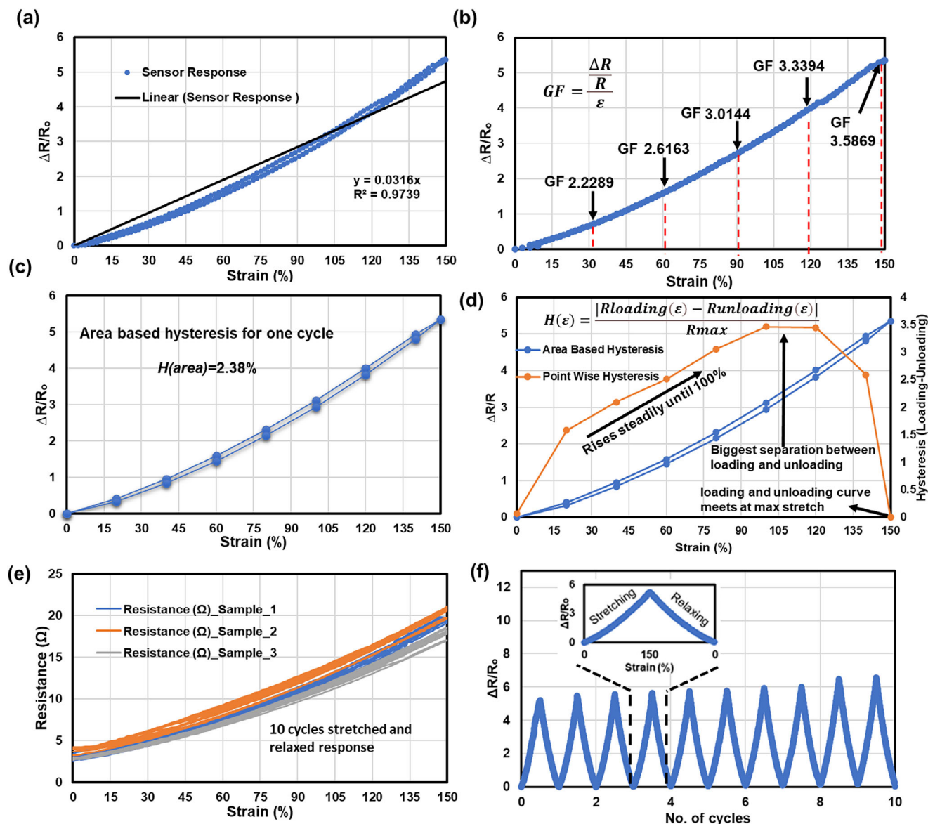
FIGURE 5 | Sensor uniaxial stretching characterization (a) Relative resistance changes as a function of strain with linear fitting and coefficient of determination. (b) Sensitivity analysis showing the calculated gauge factor across different strain ranges. (c) Hysteresis analysis for a complete cycle. (d) Hysteresis behavior during loading and unloading cycles is plotted point by point against the strain. (e) Resistance strain curves of four samples subjected to 10 repeated stretching and releasing cycles, demonstrating reproducibility. (f) Cyclic durability test up to 10 cycles, showing consistent resistance response; the inset illustrates stretching and relaxing profiles.
