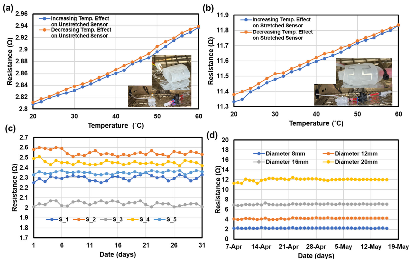
FIGURE 3 | Thermal and environmental stability of the stretchable sensors. (a,b) Temperature-dependent resistance under relaxed and stretched states. (c) Accelerated aging in a Xenon chamber, with resistance stability for various sensors during prolonged exposure. (d) Outdoor deployment of sensors with long-term resistance of sensors using a 3D pear model having varying diameters.
