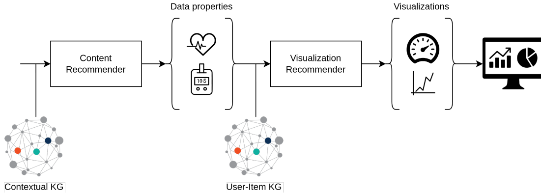
Fig. 1. Complete pipeline of the Knowledge Graph-based Context-Aware Recommender System including the input and output of the different components. The content recommender derives the most relevant data to visualize based on the context. The visualization recommender derives the best visualization type for the data based on the end-user of the dashboard.
