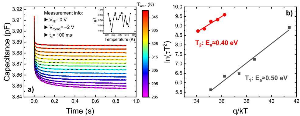
Fig. 5. a) capacitance transients captured between 285 K and 350 K applying V_{\text{fill}}=0 V, V_{\text{meas}}=-2 V, and t_p = 100 ms, together with the corresponding fits (dashed curves). The top-right inset shows the fit quality assessed via the R^2 coefficient. b) Arrhenius plot extrapolated from a). The data was fitted with a double exponential function [ y = y_0 + A_1 \exp(-t/\tau_1) + A_2 \exp(-t/\tau_2) ] to discern the two defects.
