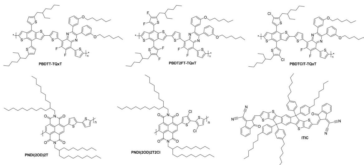
Fig. 1. Chemical structures of the donor polymers PBDTT-TQxT, PBDT2FT-TQxT and PBDDClT-TQxT, and the acceptors PNDI(2OD)2T, PNDI(2OD)2T2Cl and ITIC.
