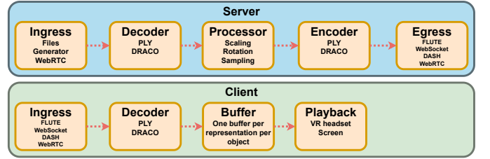
Fig. 2. Modular pipeline for real-time volumetric media.
