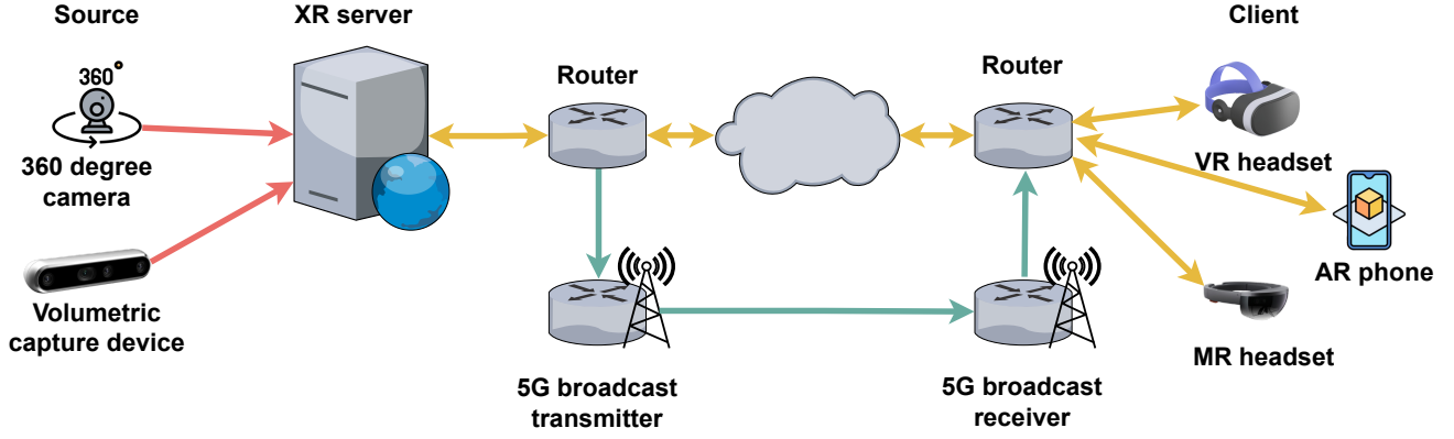
Fig. 1. End-to-end hybrid delivery concept for real-time volumetric media. Content is captured either by a 360° camera or by a volumetric capture device capable of producing point-cloud video. After processing on an XR server, the media are distributed over two complementary paths: the conventional Internet Protocol broadband network and a 5G broadcast link. The streamed scene can then be consumed on Virtual Reality headsets, Mixed Reality headsets and phones with Augmented Reality functionality.
