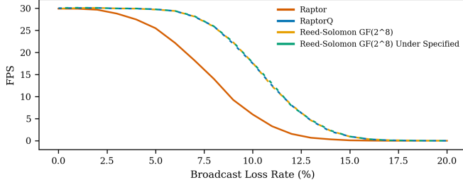
Fig. 4. Frame-rate resilience of FLUTE with 15% FEC under increasing packet-loss rates. Decoding success rate is non-linear and can be inferred from the frame-rate curve.
