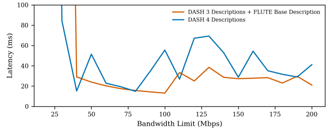
Fig. 6. Average latency of the setup for DASH as the unicast bandwidth cap is increased. Latency depends on the selected quality representation, which depends on the bandwidth cap.
