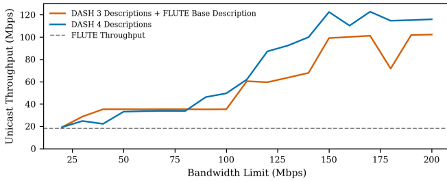
Fig. 5. Average unicast throughput of the stream in the setup as the unicast bandwidth cap is increased. The throughput used by FLUTE for transmitting the baseline quality with a bandwidth cap of 200Mbps is shown for reference.
