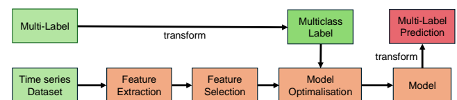
Figure 1: Pipeline with feature extraction, feature selection, and model optimization steps and multi-labels transformed into a multiclass setting for improved performance.
